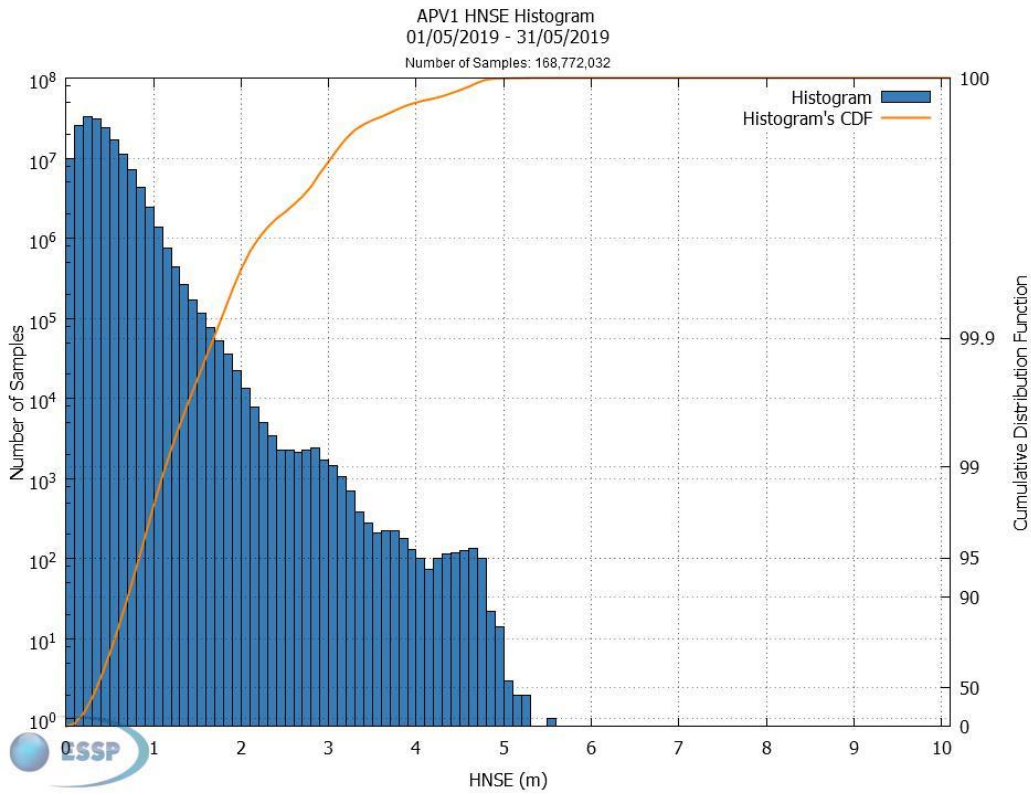
Figure 16 – EGNOS APV-I HNSE Histogram and Cumulative Probability
