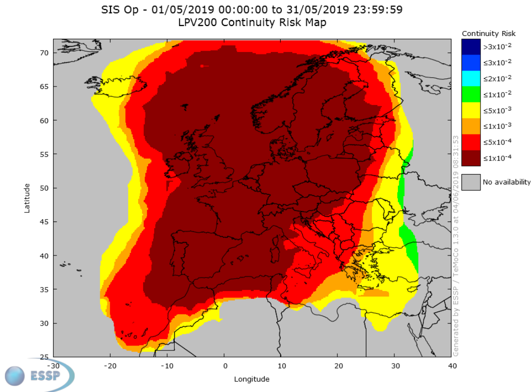
Figure 22 – EGNOS LPV-200 Continuity 2
