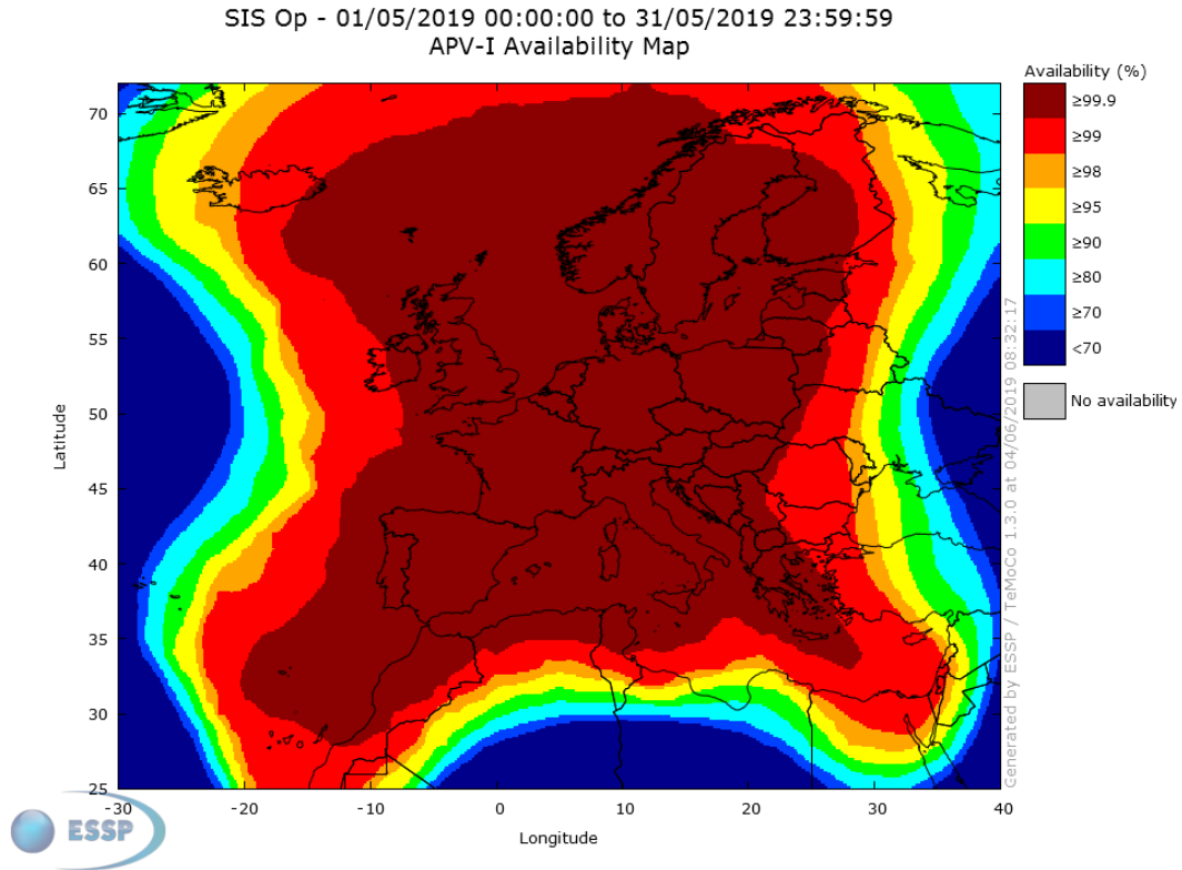
Figure 11 – EGNOS APV-I Availability
