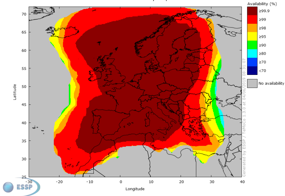
Figure 20 – EGNOS LPV-200 Availability
