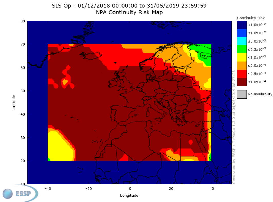
Figure 8 – EGNOS NPA Continuity over the last 6 months
