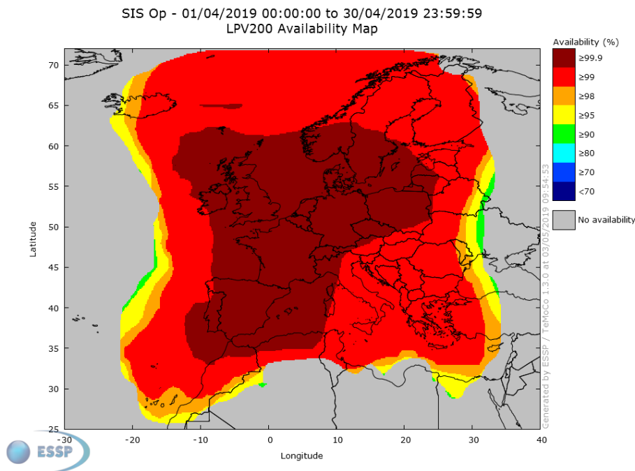
Figure 20 – EGNOS LPV-200 Availability
