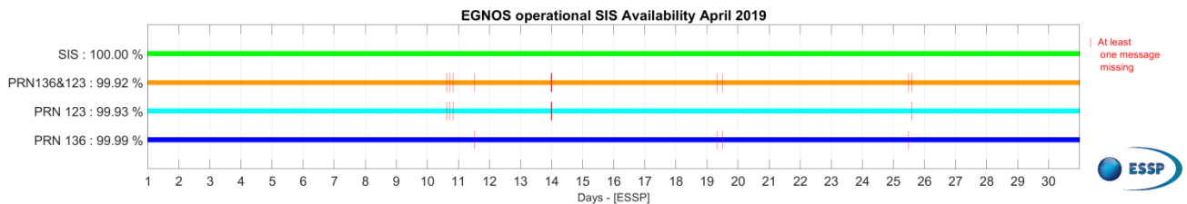
Figure 1 – EGNOS SIS & PRN Availability for April 2019.
