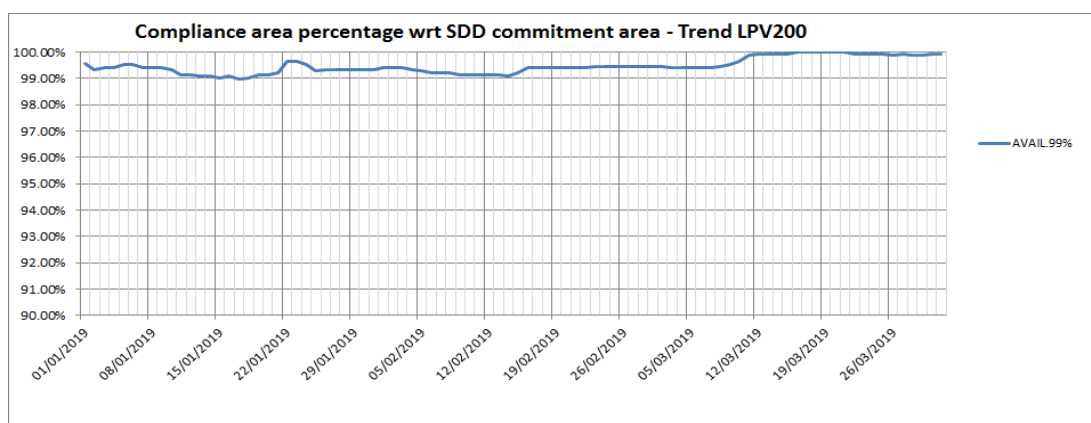
Figure 21 – EGNOS LPV-200 availability compliance trend
