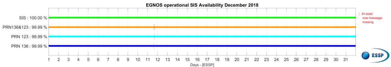
Figure 1 – EGNOS SIS & PRN Availability for December 2018.
