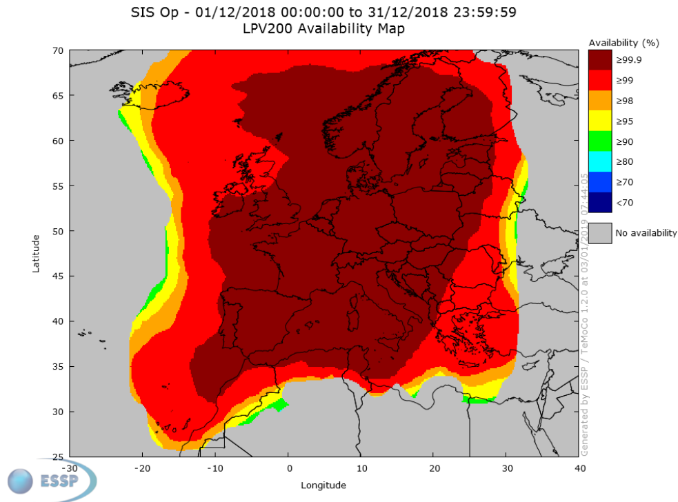
Figure 20 – EGNOS LPV-200 Availability
