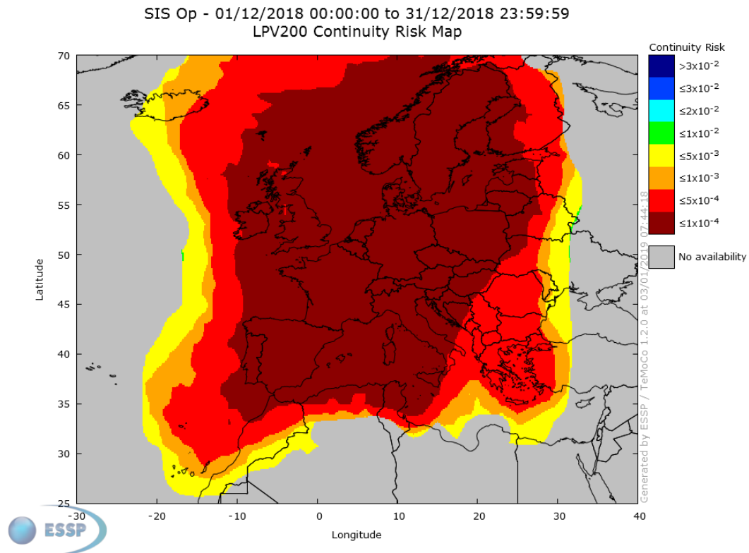
Figure 22 – EGNOS LPV-200 Continuity 3
