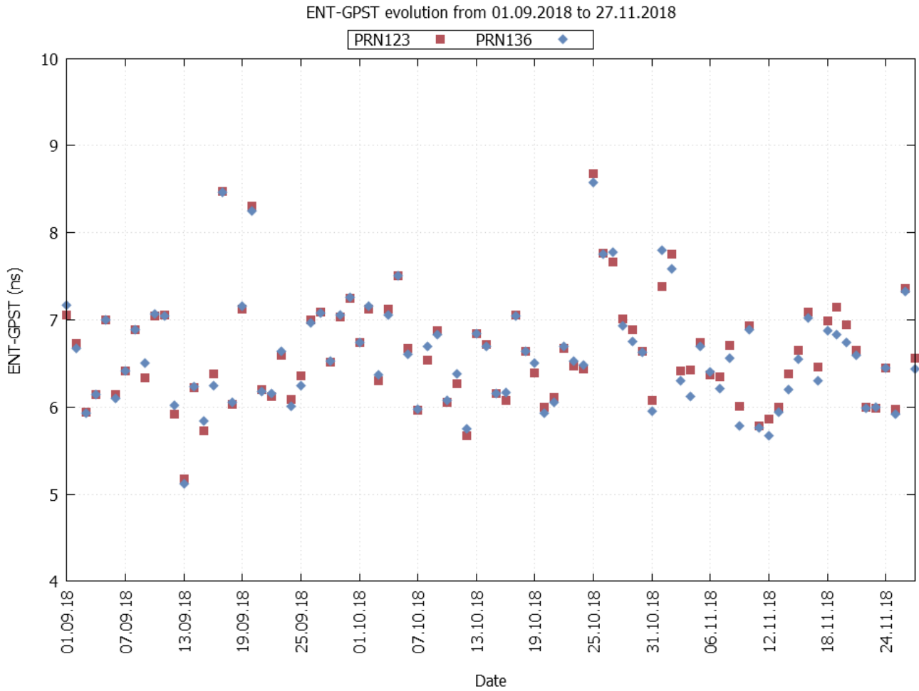
Figure 30 – ENT-GPS offset evolution
