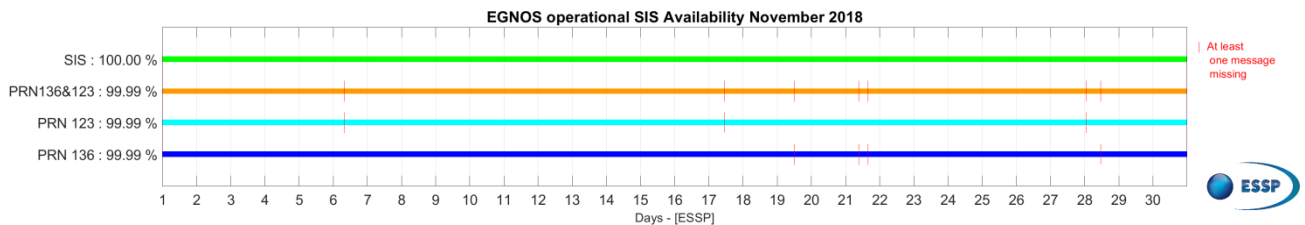
Figure 1 – EGNOS SIS & PRN Availability for November 2018.
