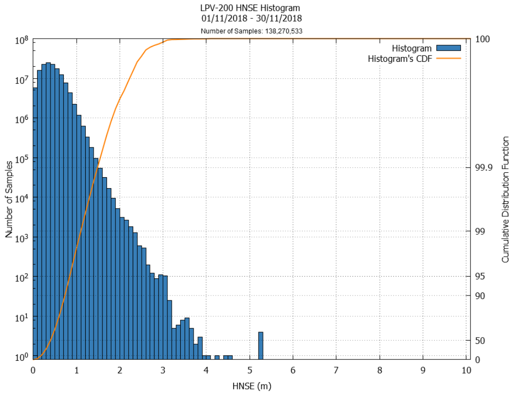
Figure 25 – EGNOS LPV-200 HNSE Histogram and Cumulative Probability
