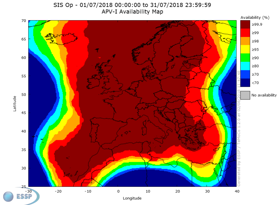
Figure 11 – EGNOS APV-I Availability
