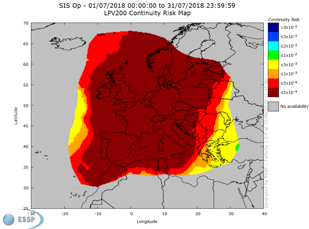
Figure 22 – EGNOS LPV-200 Continuity 2
