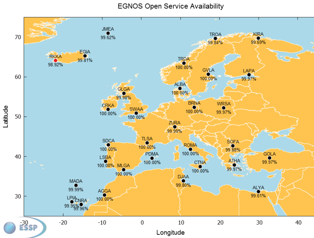
Figure 5 – EGNOS Open Service Availability at reference stations 3
