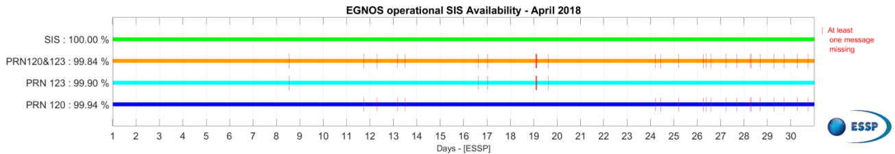
Figure 1 – EGNOS SIS & PRN Availability for April 2018.
