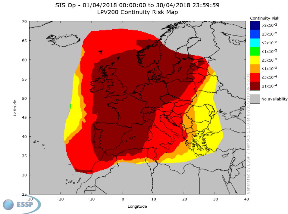
Figure 22 – EGNOS LPV-200 Continuity 6
