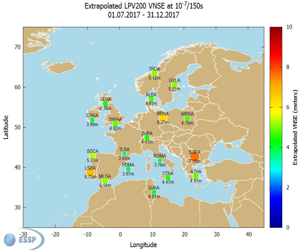
Figure 29 – Extrapolated VNSE at 10^{-7}/150s in the RIMS within the LPV200 commitment
