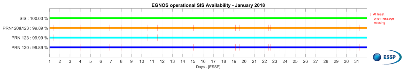
Figure 1 – EGNOS SIS & PRN Availability for January 2018.
