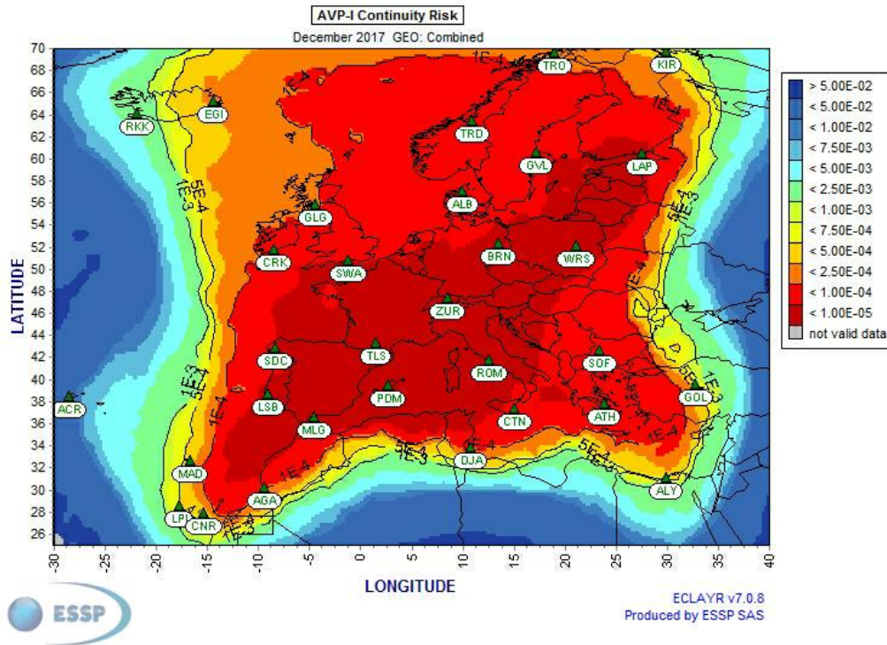
Figure 13 – EGNOS APV-I Continuity
