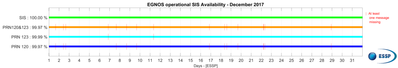
Figure 1 – EGNOS SIS & PRN Availability for December 2017.
