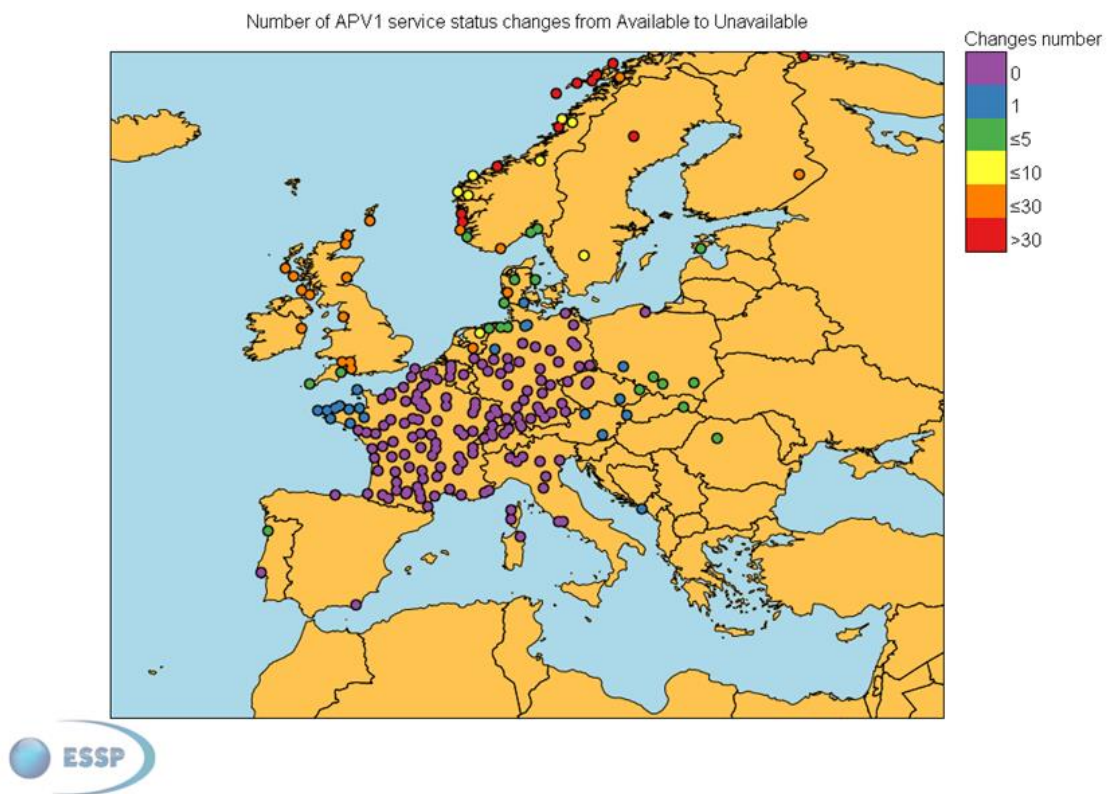
Figure 19 – EGNOS APV-I outages
