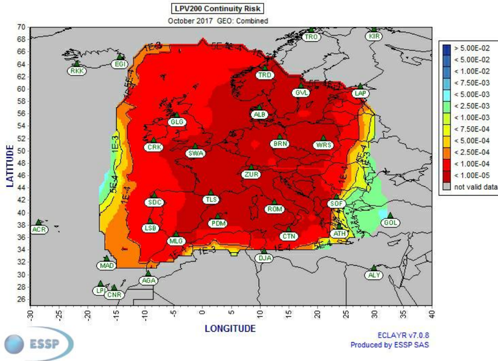
Figure 22 – EGNOS LPV-200 Continuity 3
