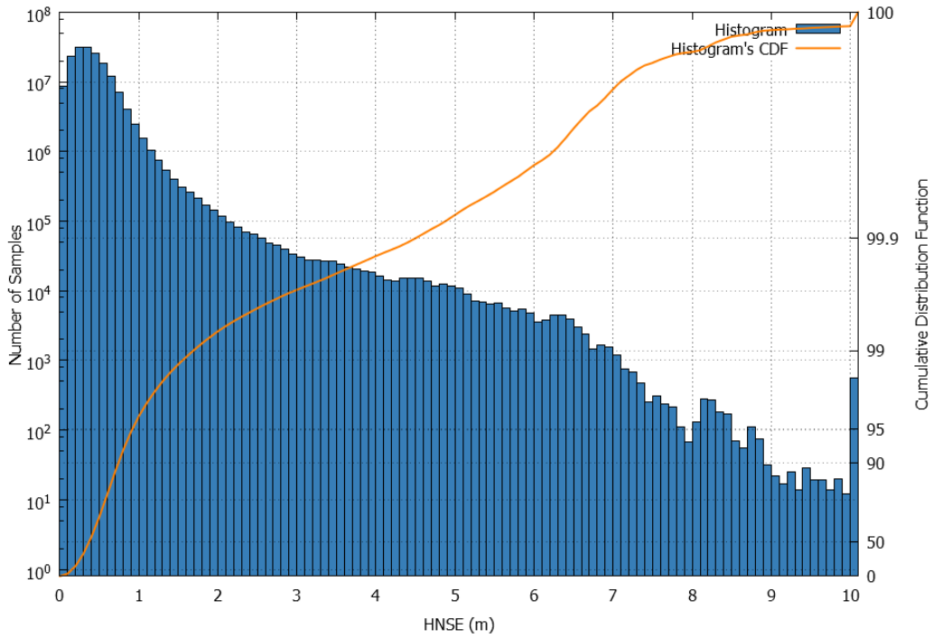
Figure 10 – EGNOS NPA HNSE Histogram and Cumulative Probability
