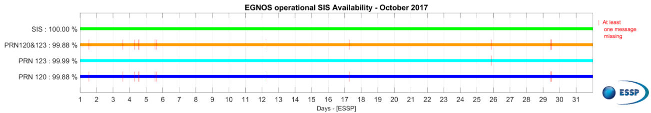
Figure 1 – EGNOS SIS & PRN Availability for October 2017.
