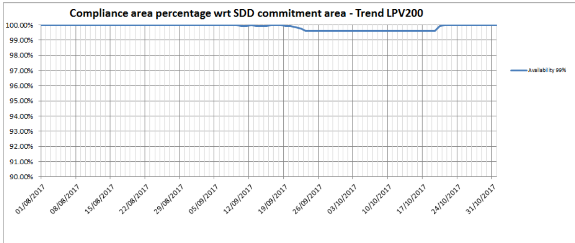
Figure 21 – EGNOS LPV-200 availability 2 compliance trend
