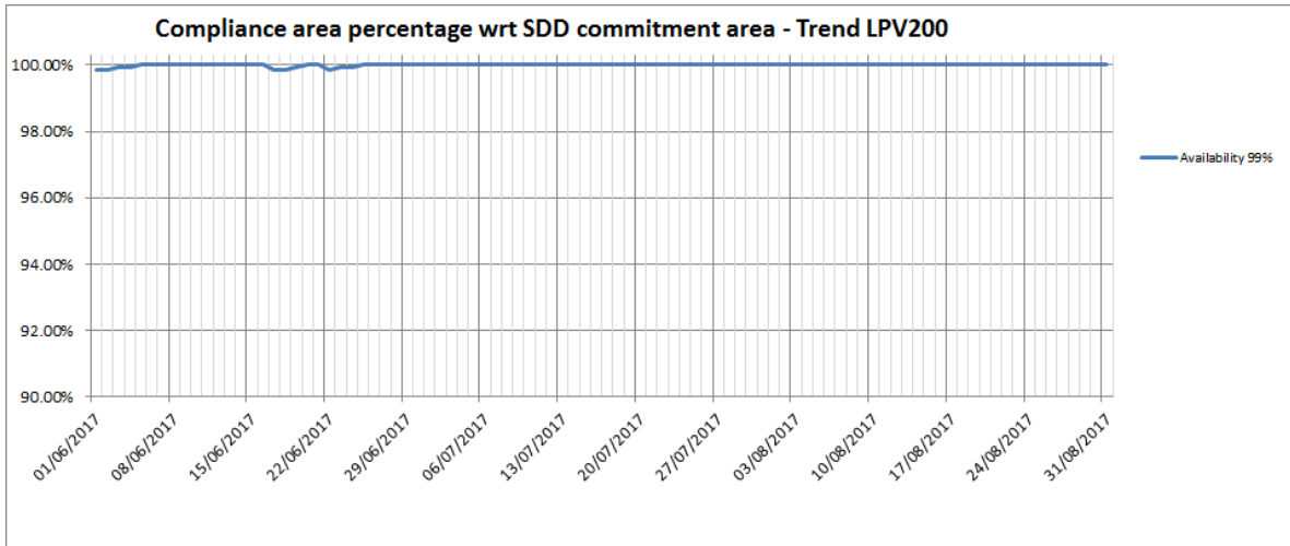
Figure 21 – EGNOS LPV-200 availability 4 compliance trend
