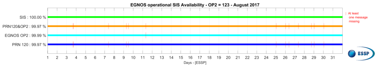
Figure 1 – EGNOS SIS & PRN Availability for August 2017.
