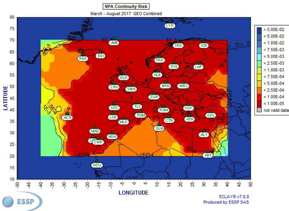
Figure 8 – EGNOS NPA Continuity over the last 6 months 3
