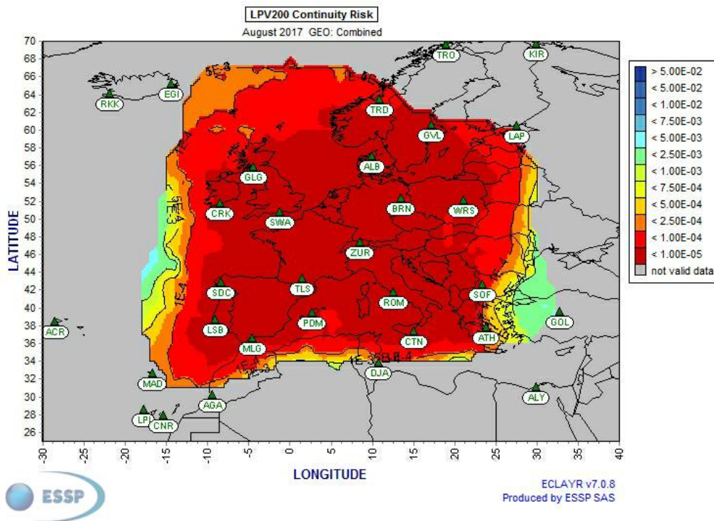
Figure 22 – EGNOS LPV-200 Continuity 5
