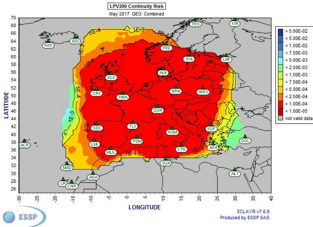
Figure 22 – EGNOS LPV-200 Continuity 8
