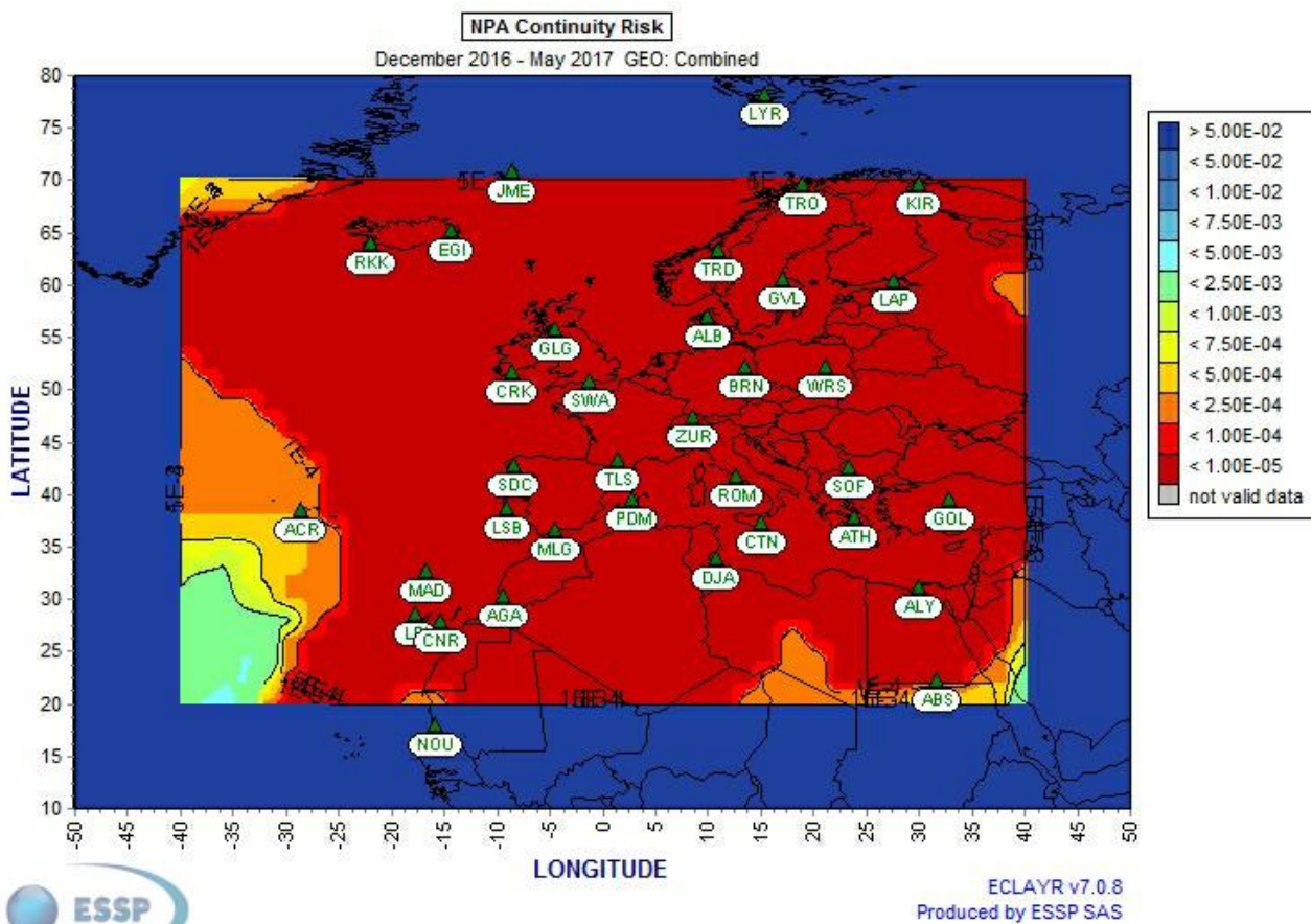
Figure 8 – EGNOS NPA Continuity over the last 6 months 4
