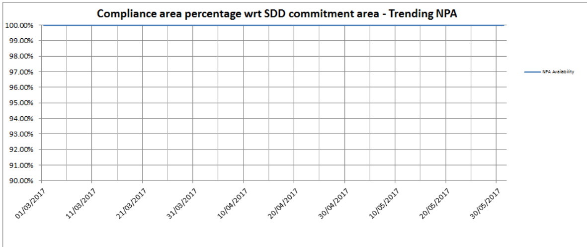
Figure 7 – EGNOS NPA availability 3 compliance trend
