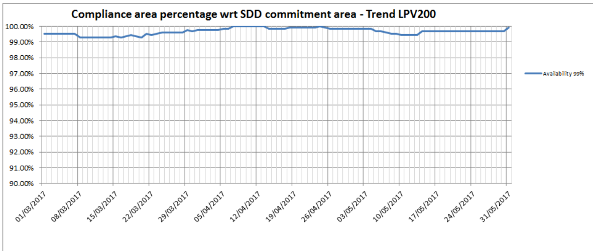
Figure 21 – EGNOS LPV-200 availability 6-7 compliance trend
