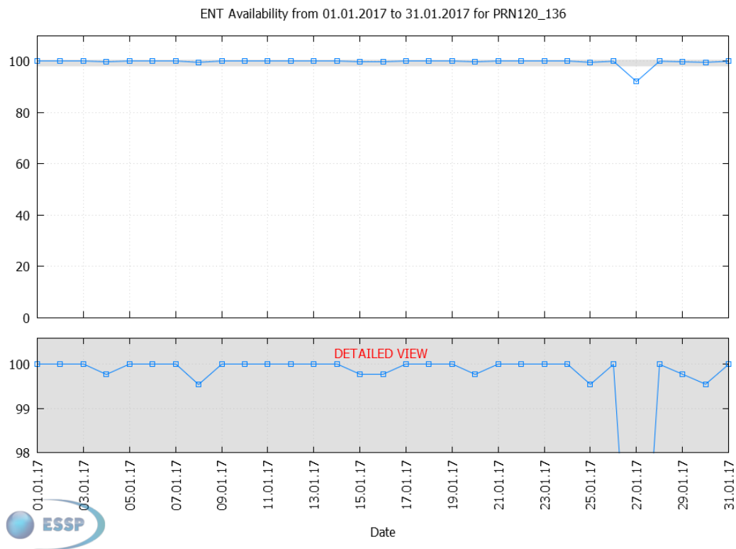
Figure 30 – EGNOS Time Service availability
