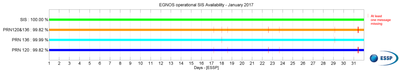
Figure 1 – EGNOS SIS & PRN Availability for January 2017.
