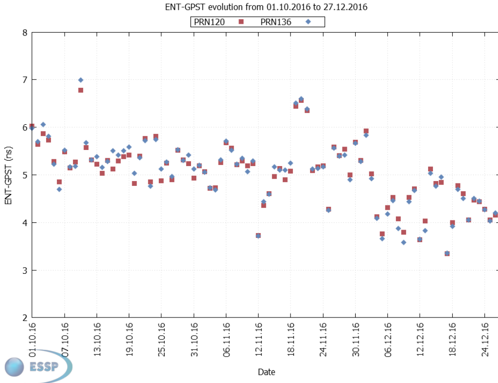
Figure 31 – ENT-GPS offset evolution
