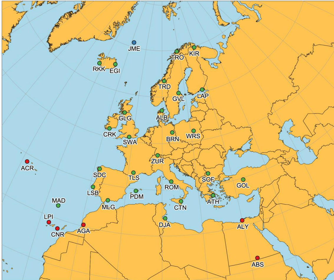
Figure 32 – EGNOS RIMS sites used in this report
