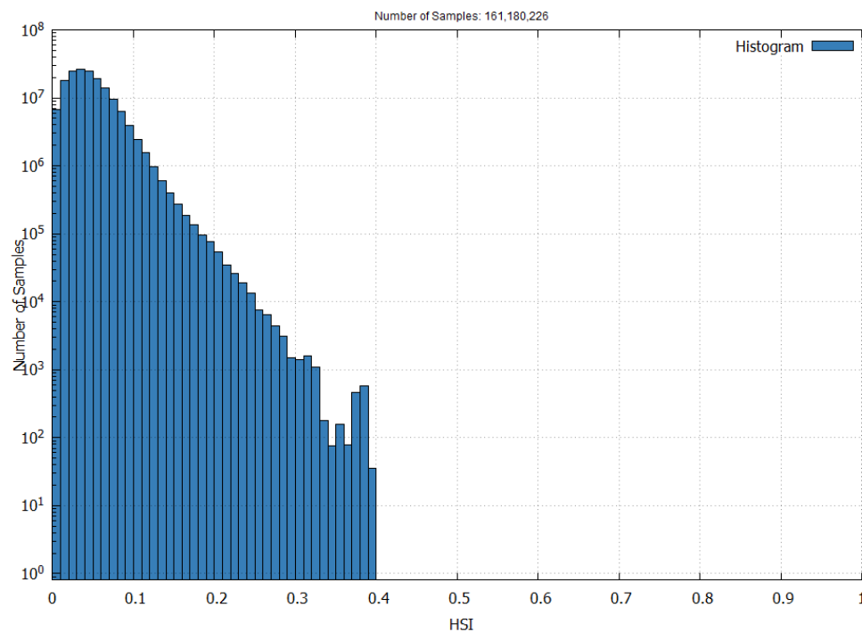
Figure 8 – EGNOS NPA Horizontal Safety Index in September 2026
