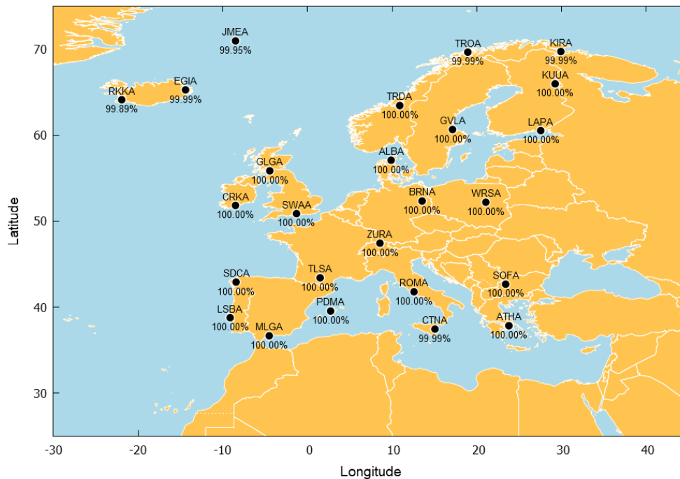
Figure 5 – EGNOS Open Service Availability at reference stations in September 2026
