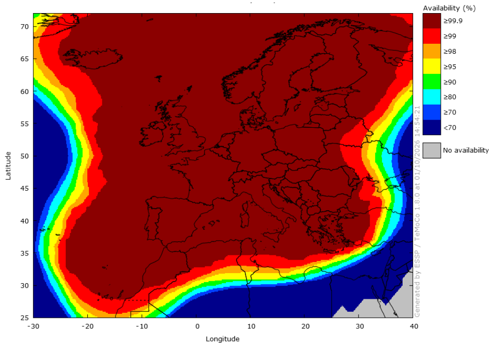
Figure 10 – EGNOS APV-I Availability in September 2026
