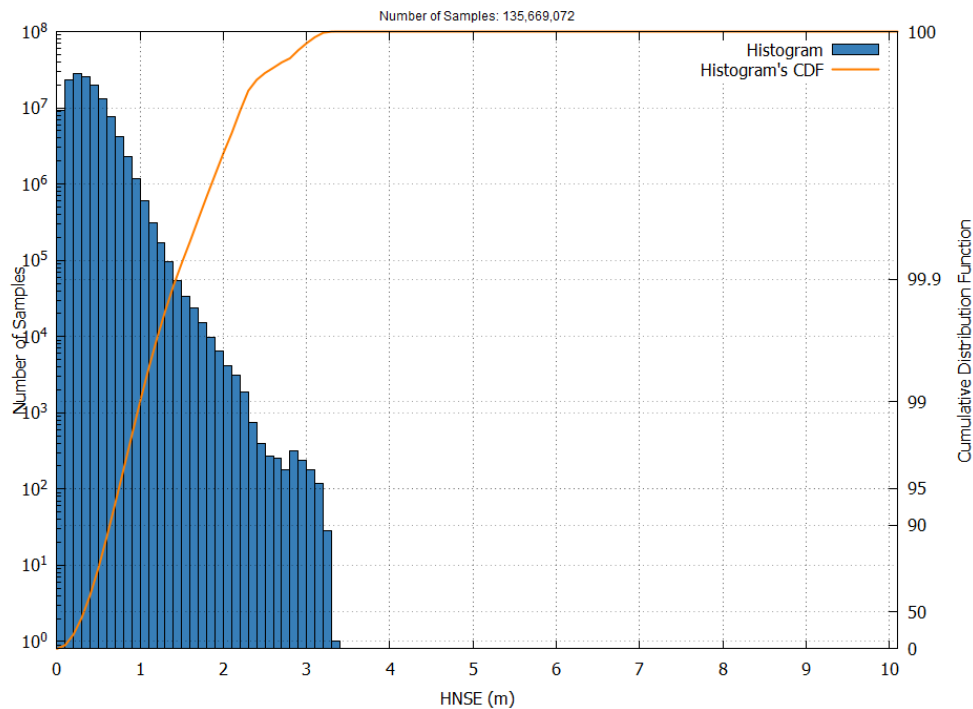
Figure 24 – EGNOS LPV-200 HNSE Histogram and Cumulative Probability in September 2026
