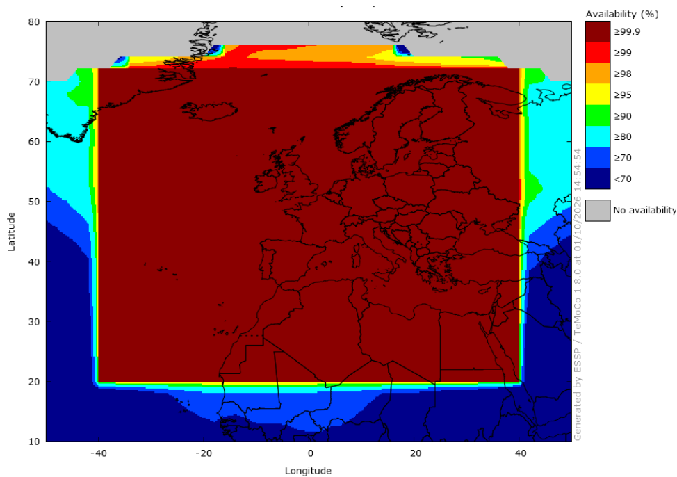
Figure 6 – EGNOS NPA Availability in September 2026
