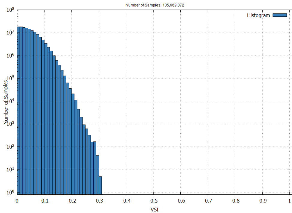
Figure 23 – EGNOS LPV-200 Vertical Safety Index in September 2026
