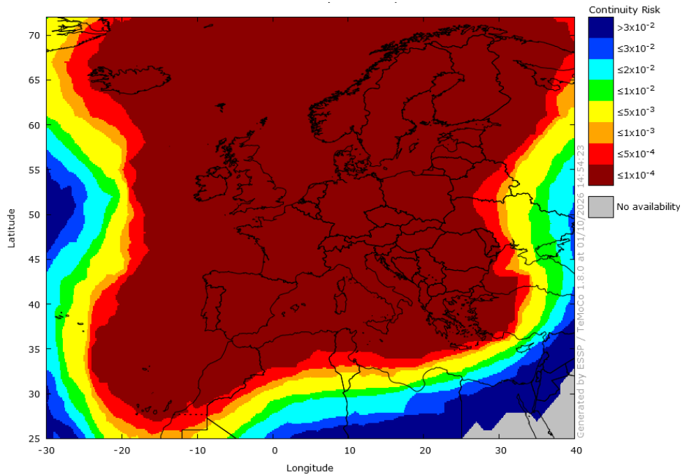
Figure 12 – EGNOS APV-I Continuity in September 2026
