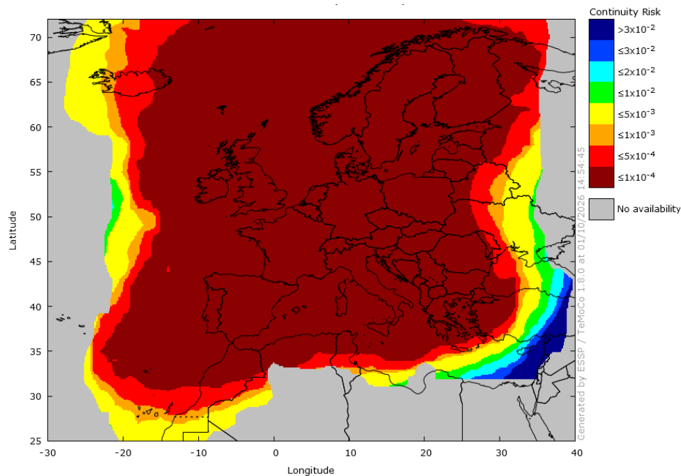
Figure 21 – EGNOS LPV-200 Continuity 2 in September 2026
