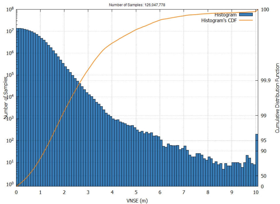
Figure 4 – EGNOS Open Service VNSE Histogram and Cumulative Probability in September 2026
