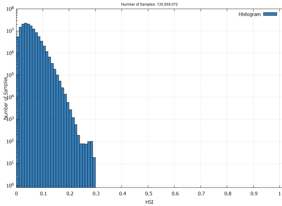
Figure 22 – EGNOS LPV-200 Horizontal Safety Index in September 2026
