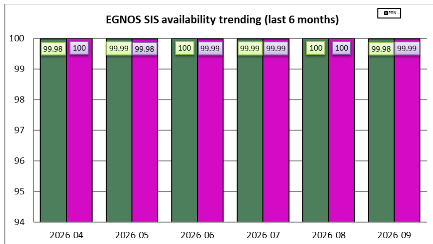
Figure 2 – Trend of EGNOS SIS Availability per GEO for the past 6 months (in green PRN 136; in purple PRN 121)
