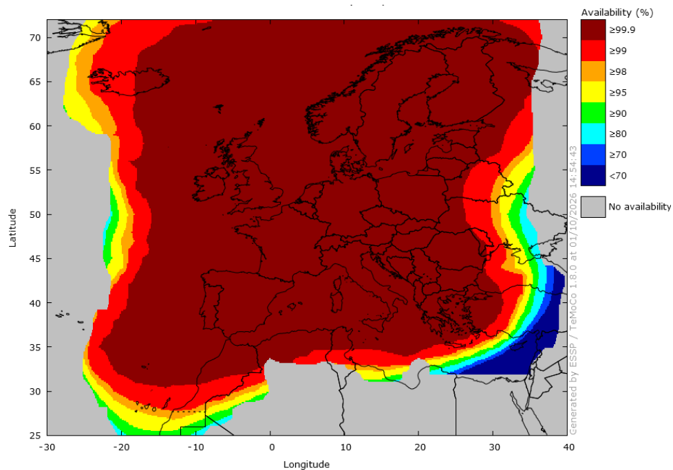
Figure 19 – EGNOS LPV-200 Availability in September 2026
