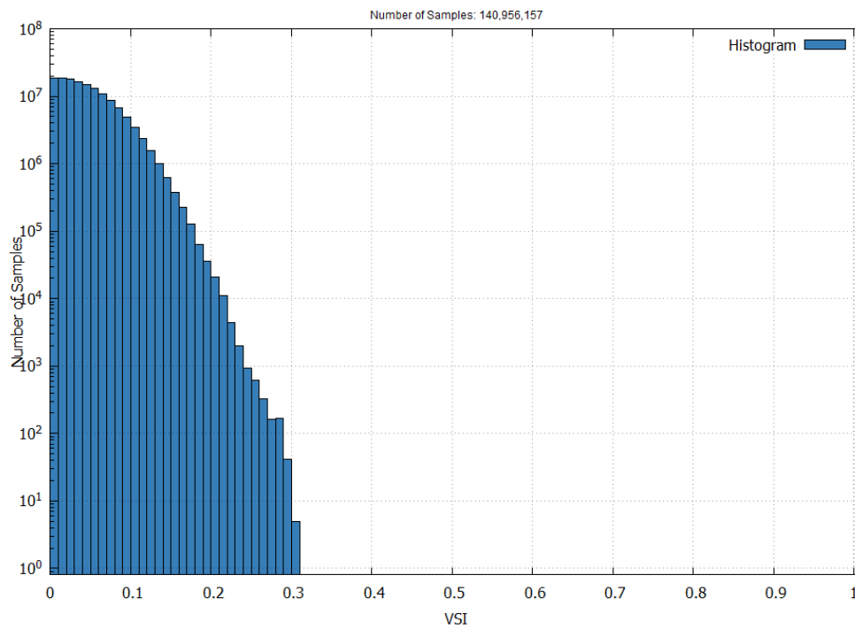
Figure 14 – EGNOS APV-I Vertical Safety Index in September 2026
