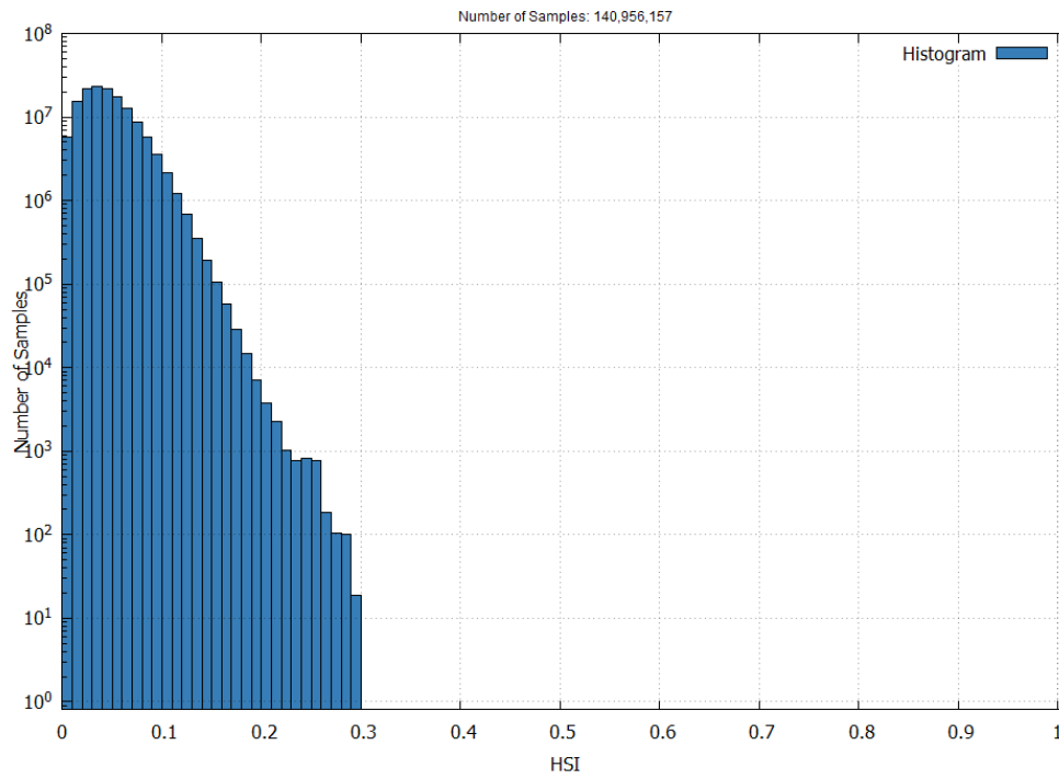
Figure 13 – EGNOS APV-I Horizontal Safety Index in September 2026
