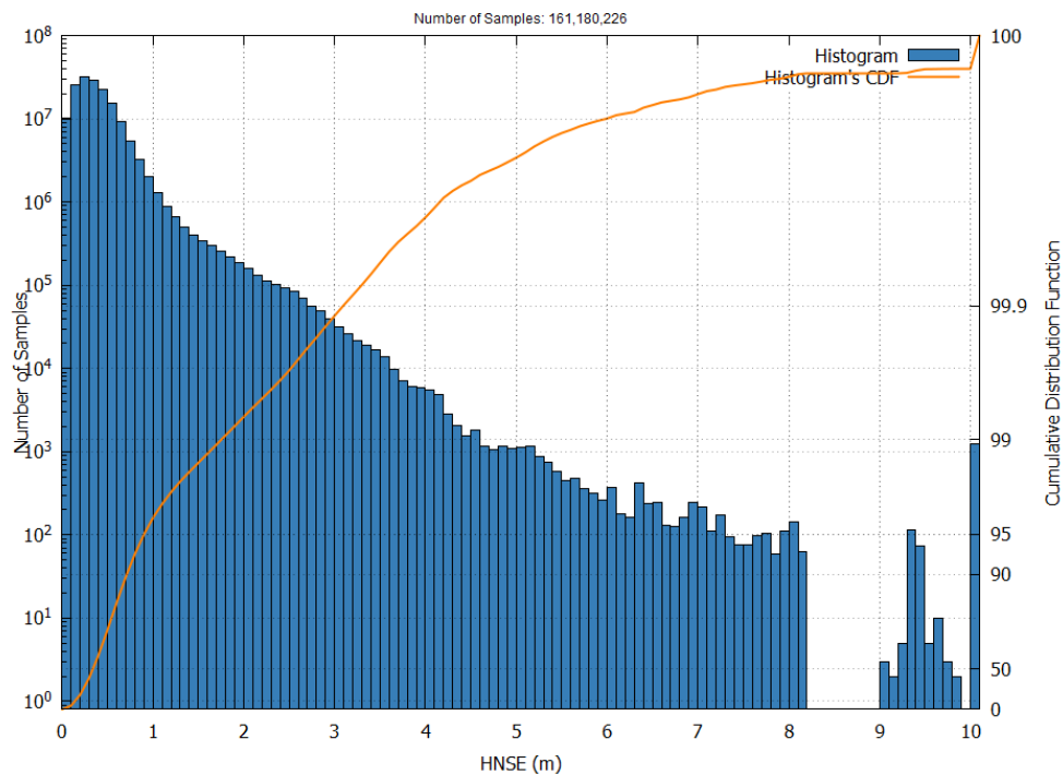
Figure 9 – EGNOS NPA HNSE Histogram and Cumulative Probability in September 2026
