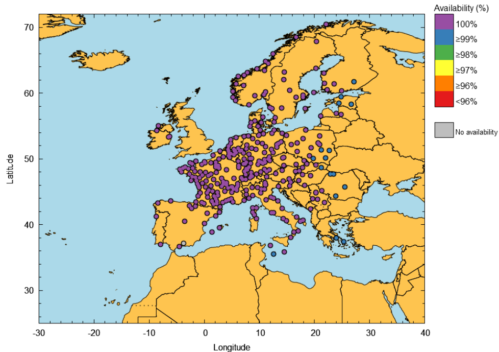
Figure 27 – EGNOS LPV-200 Availability at airports in September 2026
