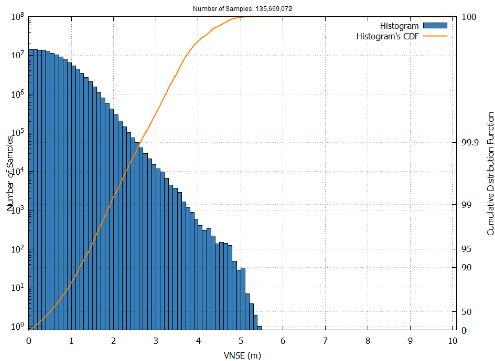
Figure 25 – EGNOS LPV-200 VNSE Histogram and Cumulative Probability in September 2026
