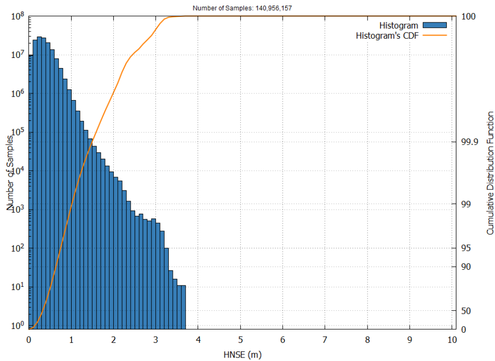
Figure 15 – EGNOS APV-I HNSE Histogram and Cumulative Probability in September 2026
