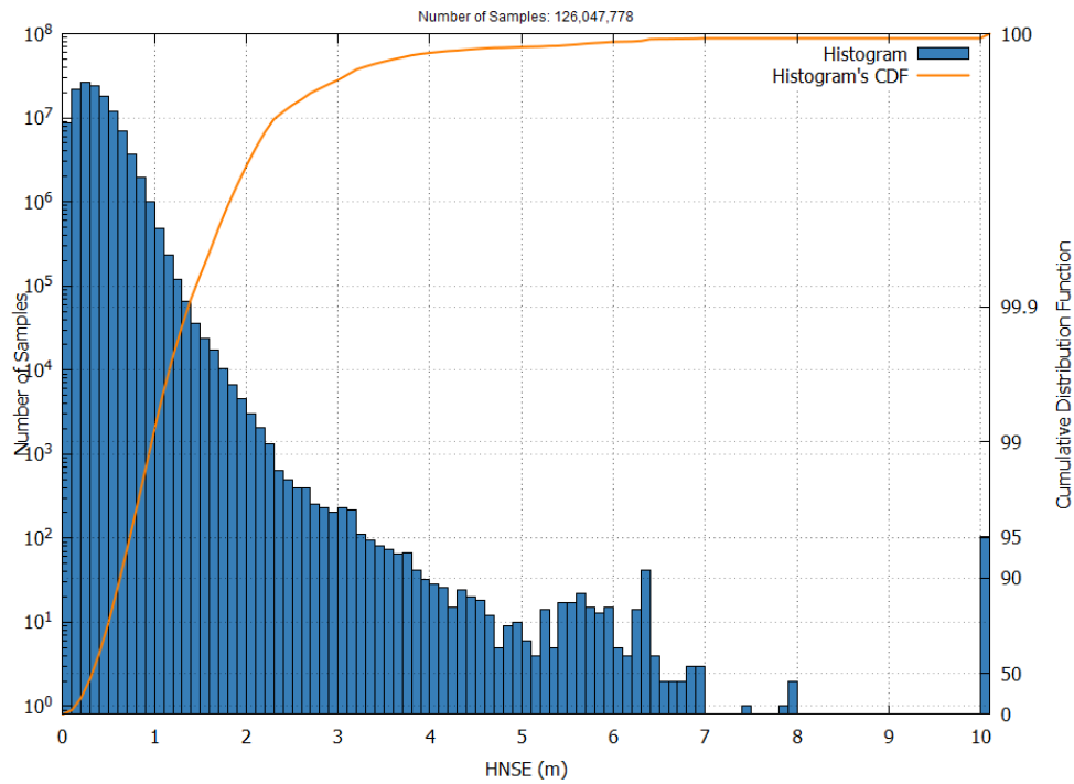
Figure 3 – EGNOS Open Service HNSE Histogram and Cumulative Probability in September 2026
