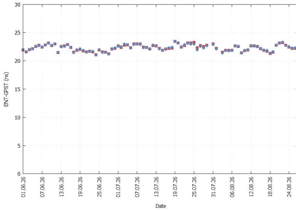
Figure 30 – ENT-GPS offset evolution from June 2026 to August 2026 (red PRN 121; blue PRN 136)
