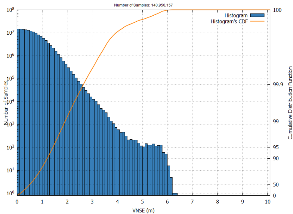
Figure 16 – EGNOS APV-I VNSE Histogram and Cumulative Probability in September 2026
