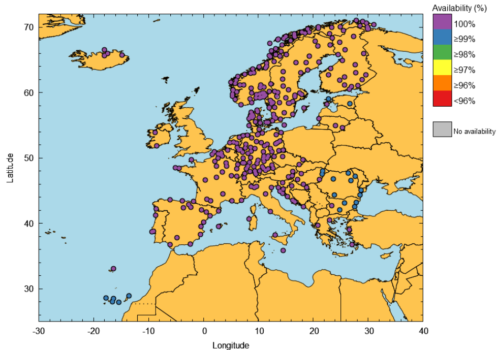
Figure 17 – EGNOS APV-I Availability at airports in September 2026
