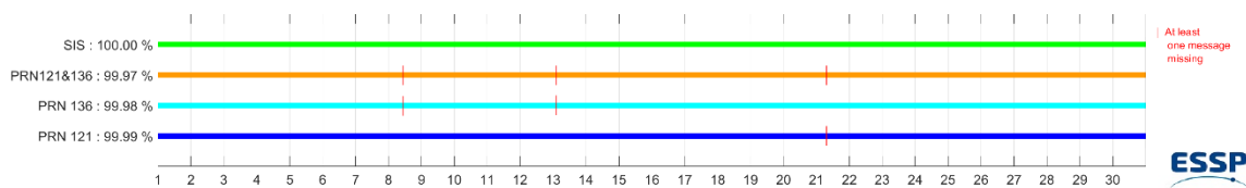
Figure 1 - EGNOS SIS & PRN Availability for September 2026
