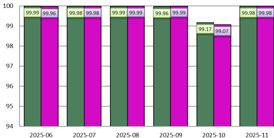
Figure 2 – Trend of EGNOS SIS Availability per GEO for the past 6 months (in green PRN 136; in purple PRN 123 until 8th September and PRN 121 from September 9th)
