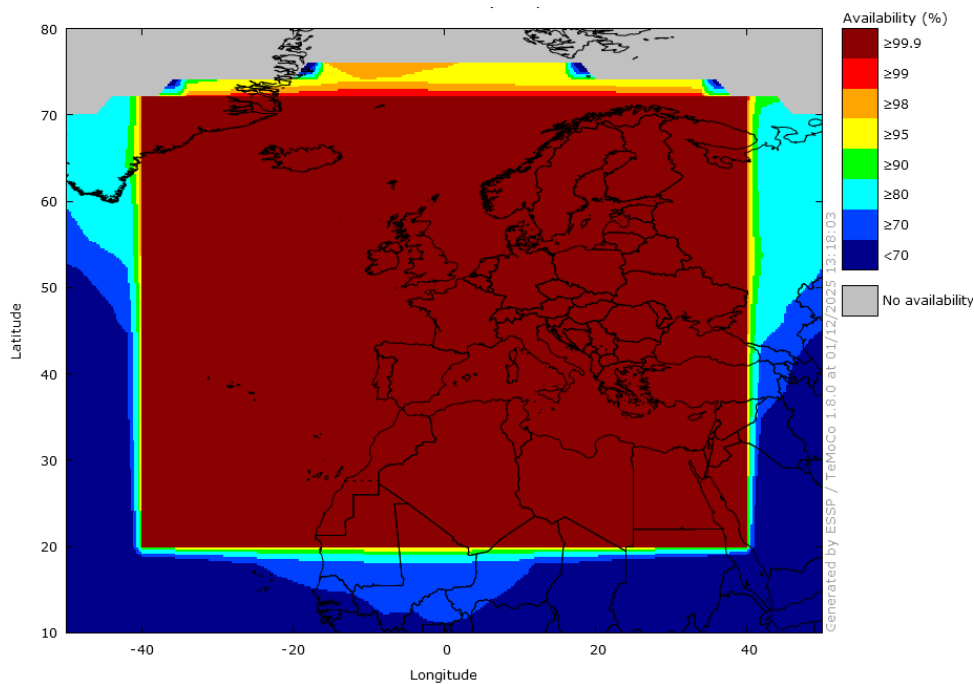
Figure 6 – EGNOS NPA Availability in November 2025
