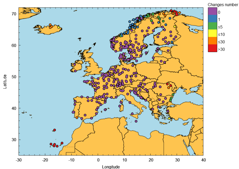
Figure 18 – EGNOS APV-I outages in November 2025
