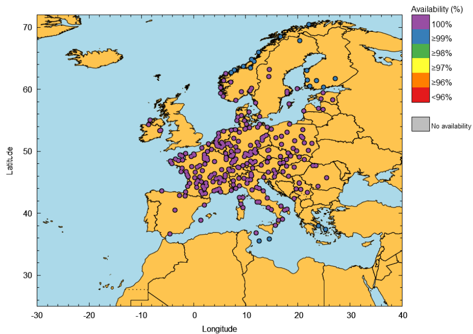
Figure 27 – EGNOS LPV-200 Availability at airports in November 2025
