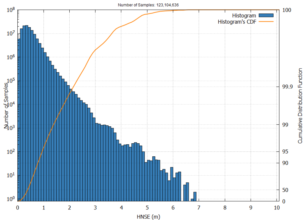
Figure 15 – EGNOS APV-I HNSE Histogram and Cumulative Probability in November 2025
