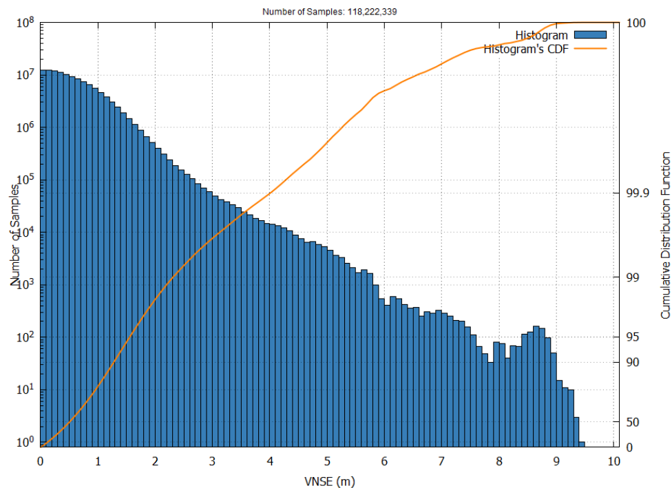
Figure 25 – EGNOS LPV-200 VNSE Histogram and Cumulative Probability in November 2025
