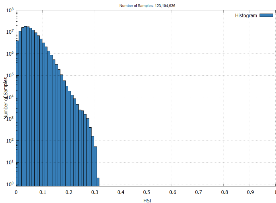
Figure 13 – EGNOS APV-I Horizontal Safety Index in November 2025
