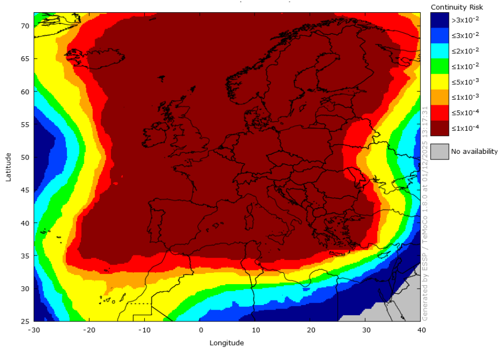
Figure 12 – EGNOS APV-I Continuity in November 2025
