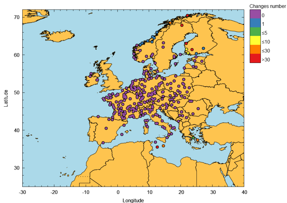
Figure 28 – EGNOS LPV-200 outages in November 2025
