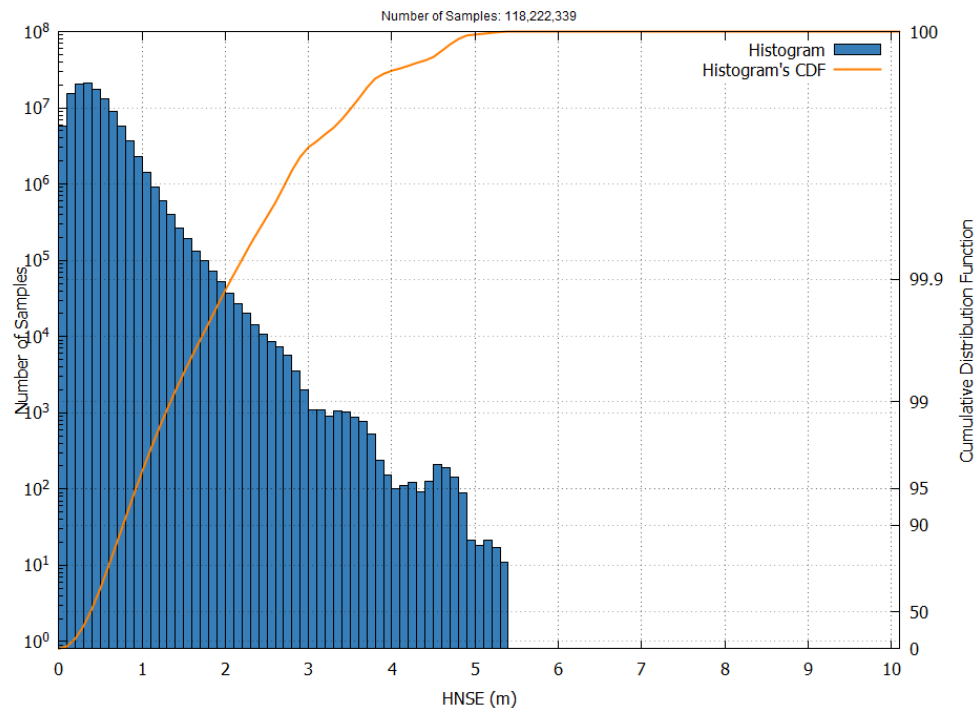
Figure 24 – EGNOS LPV-200 HNSE Histogram and Cumulative Probability in November 2025
