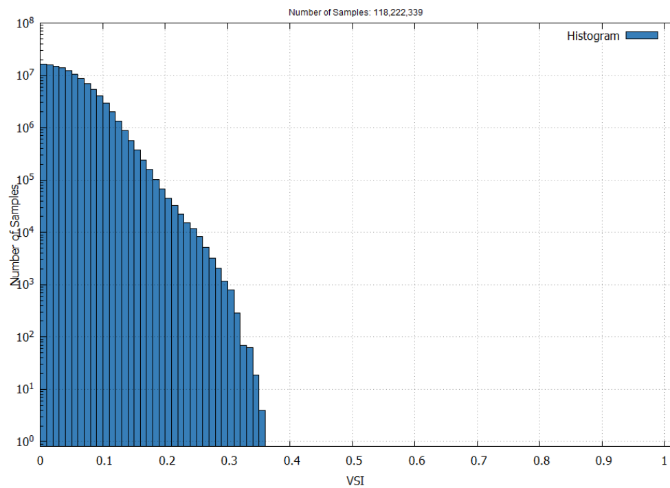
Figure 23 – EGNOS LPV-200 Vertical Safety Index in November 2025
