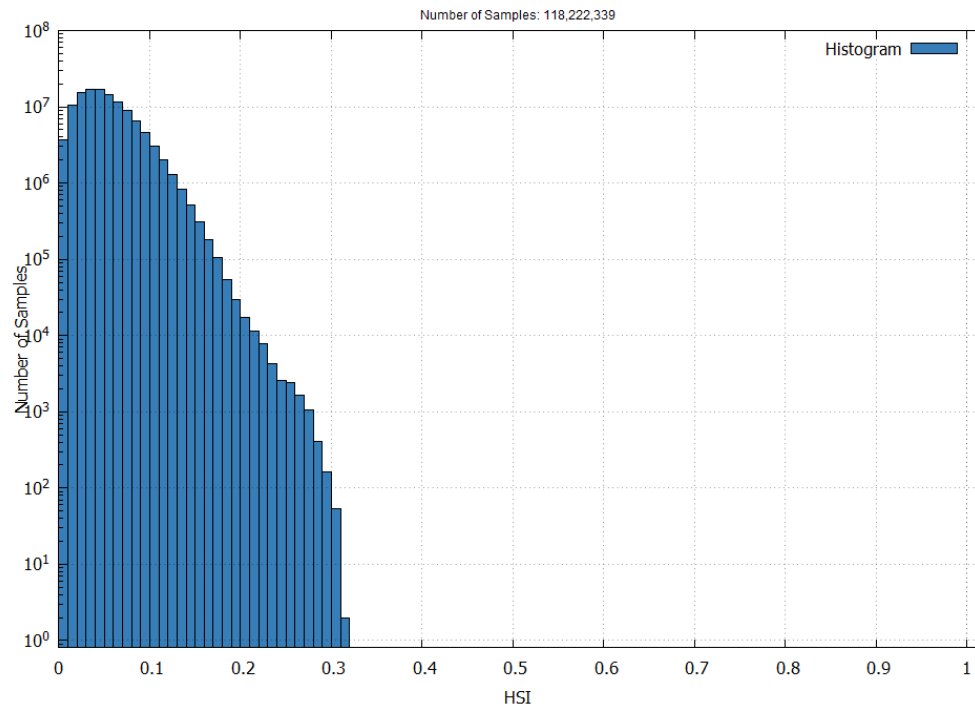
Figure 22 – EGNOS LPV-200 Horizontal Safety Index in November 2025
