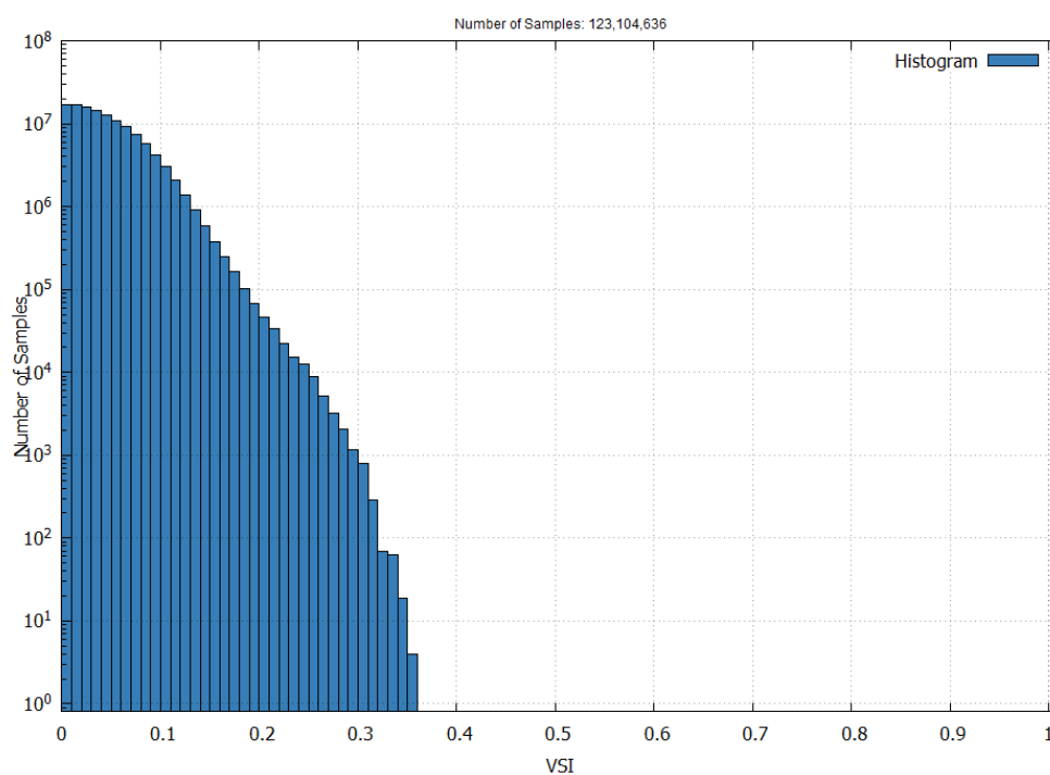
Figure 14 – EGNOS APV-I Vertical Safety Index in November 2025
