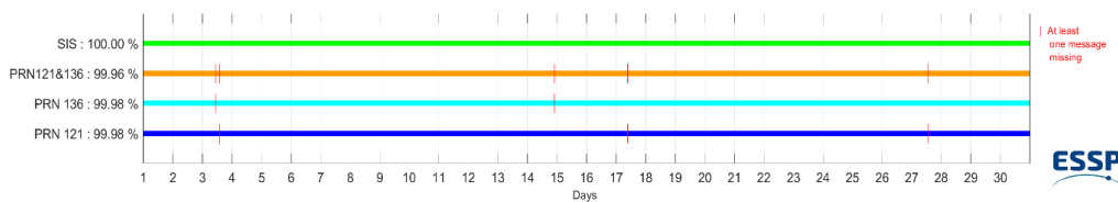
Figure 1 - EGNOS SIS & PRN Availability for November 2025
