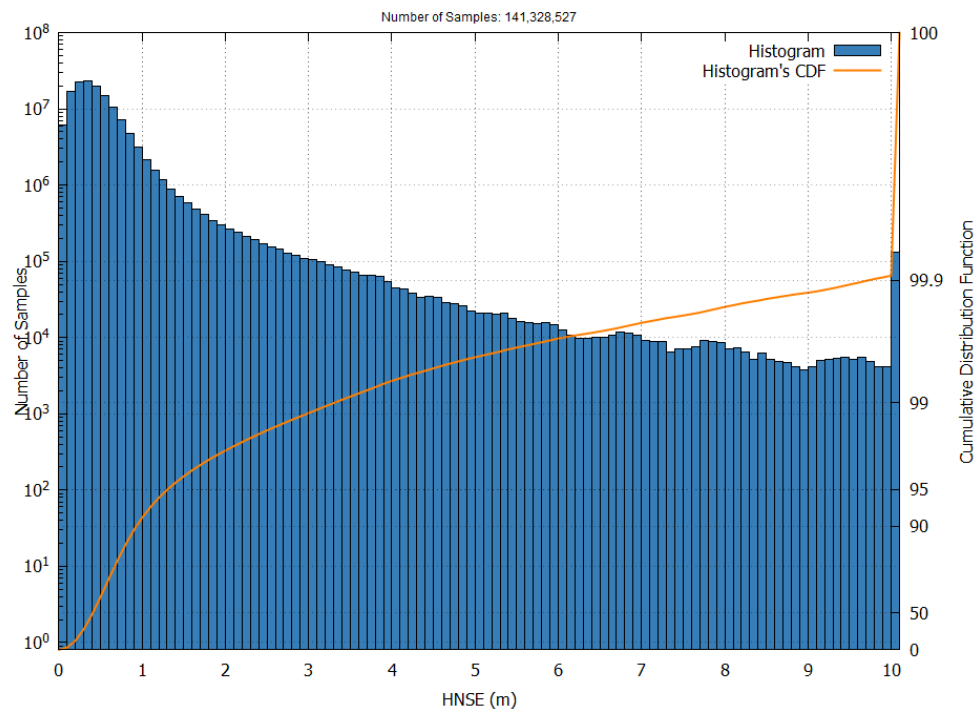
Figure 9 – EGNOS NPA HNSE Histogram and Cumulative Probability in November 2025
