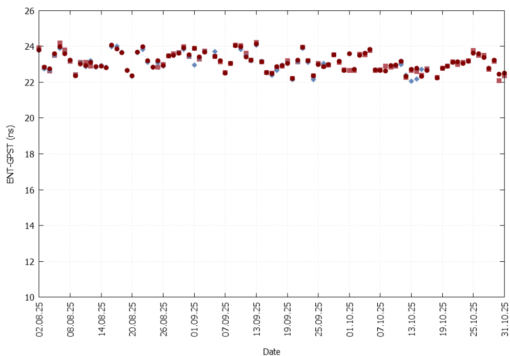
Figure 30 – ENT-GPS offset evolution from August to October 2025 (red square for PRN121, red circle for PRN136 and blue for PRN123)
