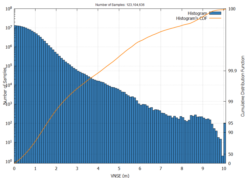
Figure 16 – EGNOS APV-I VNSE Histogram and Cumulative Probability in November 2025
