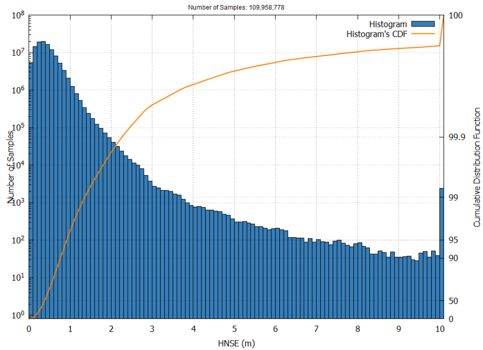
Figure 3 – EGNOS Open Service HNSE Histogram and Cumulative Probability in November 2025
