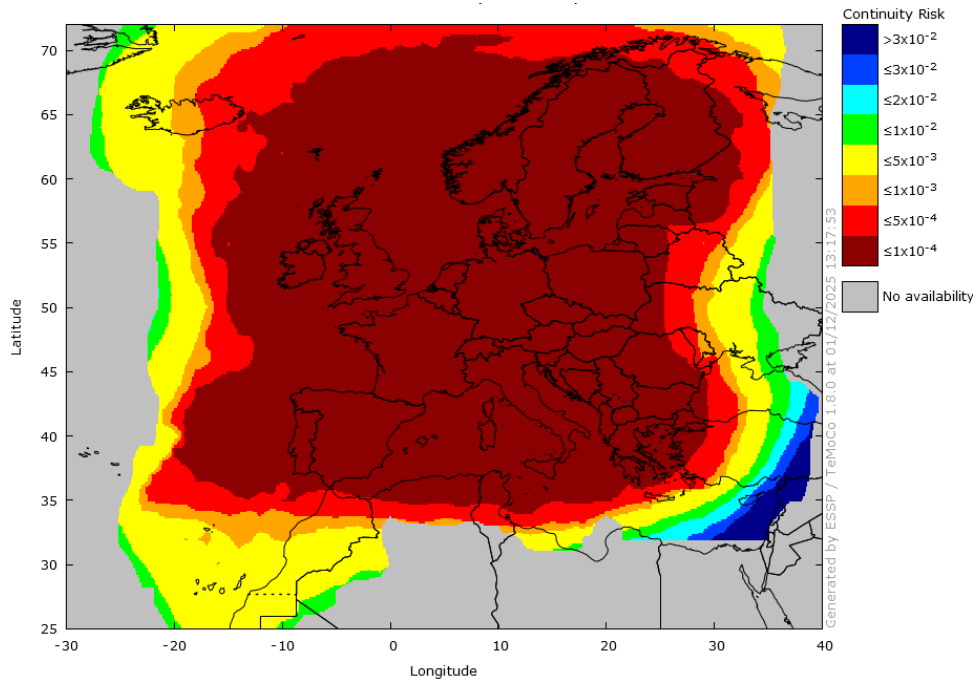
Figure 21 – EGNOS LPV-200 Continuity 2 in November 2025
