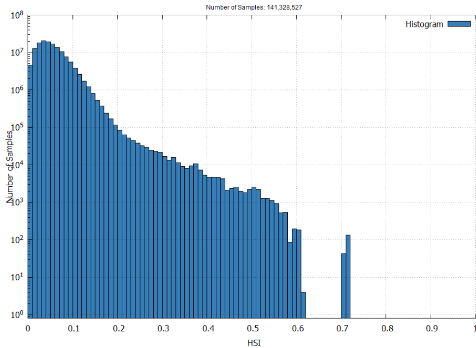
Figure 8 – EGNOS NPA Horizontal Safety Index in November 2025
