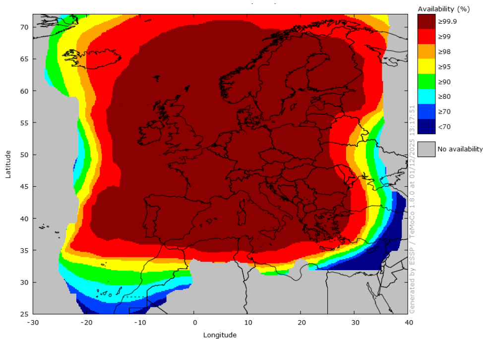
Figure 19 – EGNOS LPV-200 Availability in November 2025
