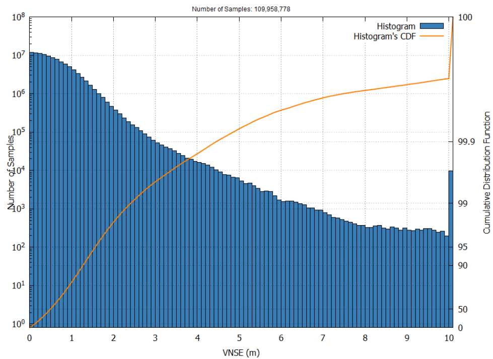
Figure 4 – EGNOS Open Service VNSE Histogram and Cumulative Probability in November 2025
