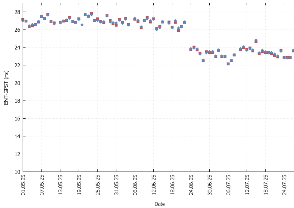
Figure 30 – ENT-GPS offset evolution from May to July 2025 (red PRN 123; blue PRN 136)
