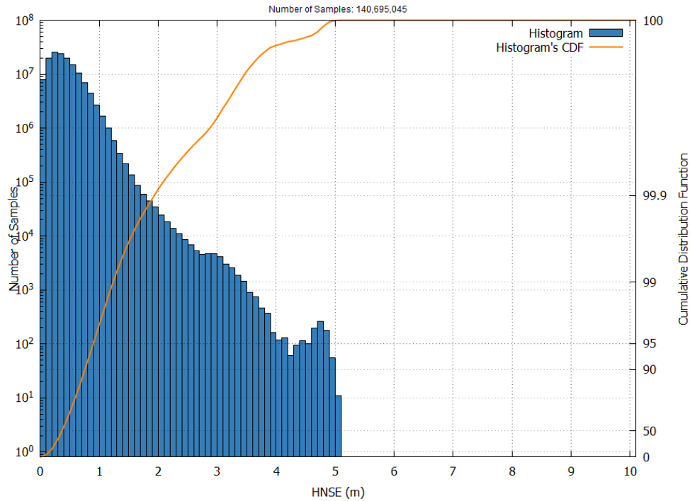
Figure 24 – EGNOS LPV-200 HNSE Histogram and Cumulative Probability in August 2025
