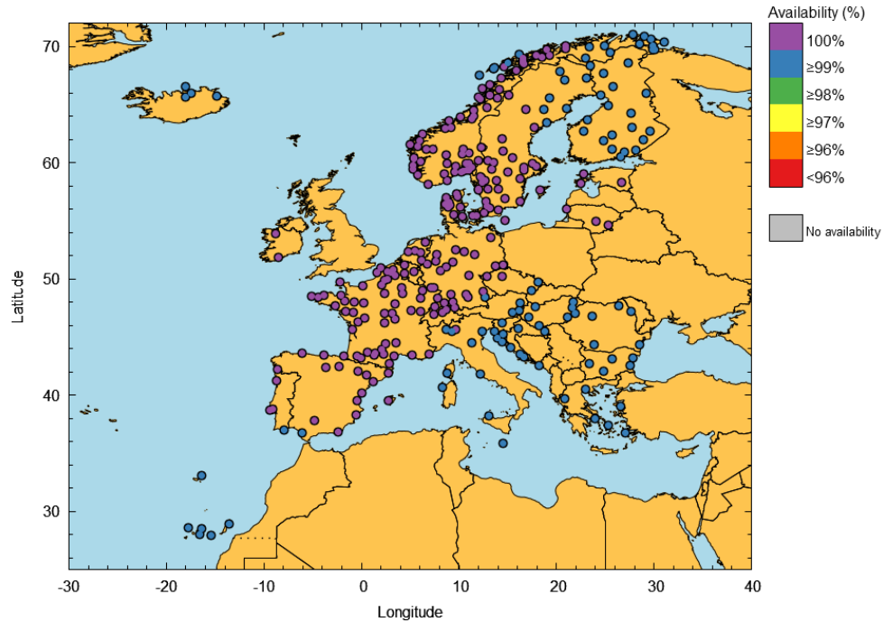
Figure 17 – EGNOS APV-I Availability at airports in August 2025
