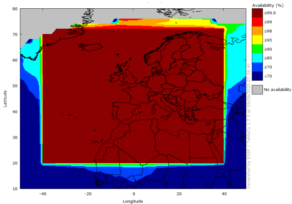
Figure 6 – EGNOS NPA Availability in August 2025
