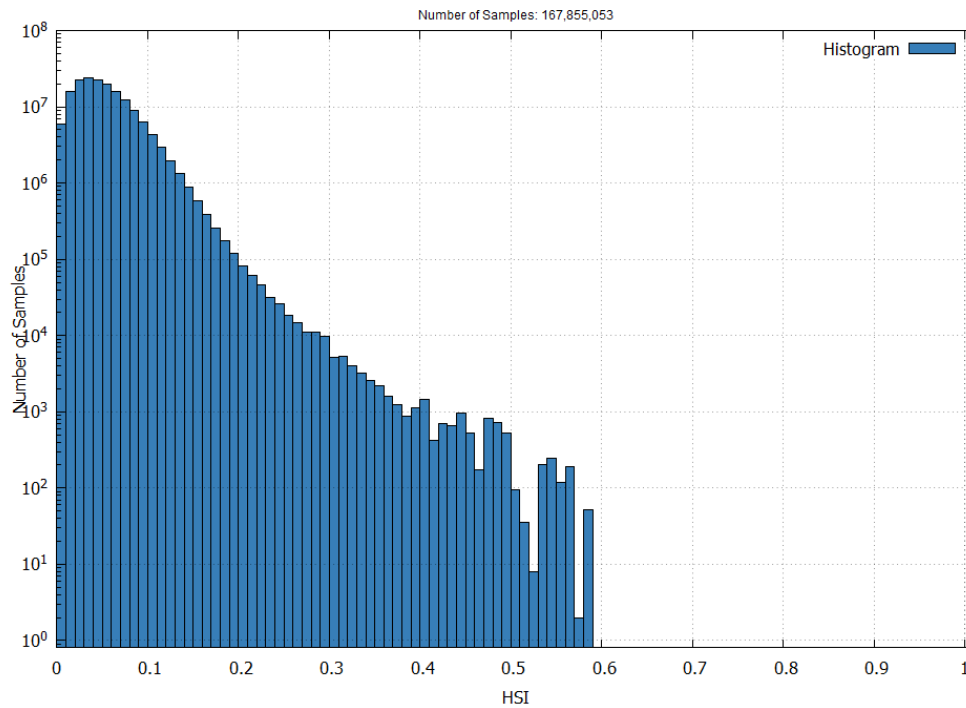
Figure 8 – EGNOS NPA Horizontal Safety Index in August 2025
