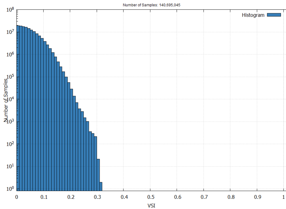
Figure 23 – EGNOS LPV-200 Vertical Safety Index in August 2025
