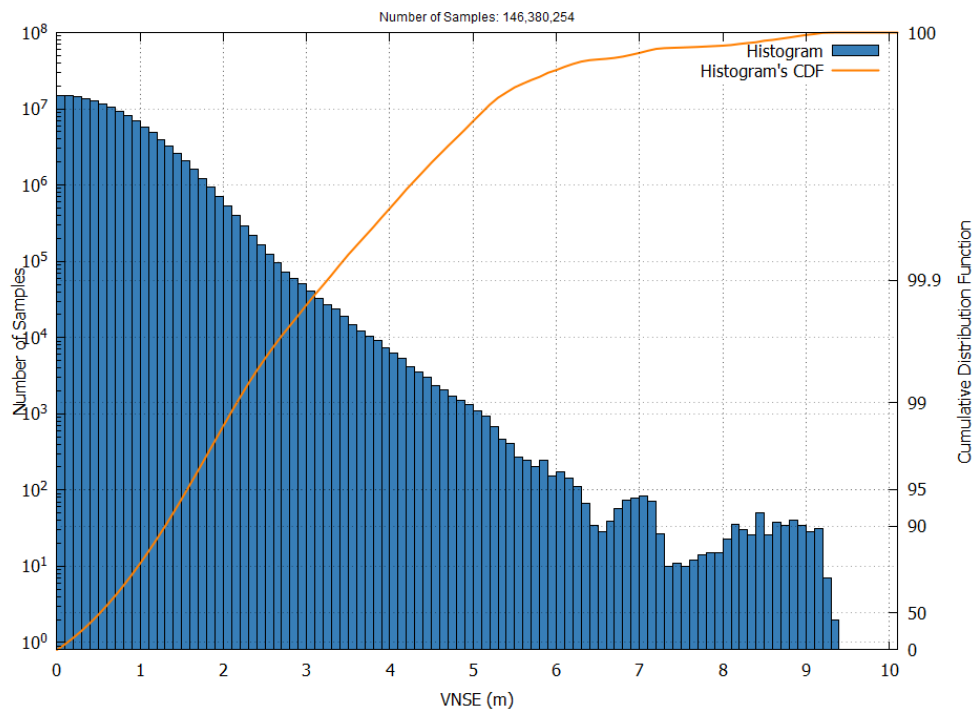
Figure 16 – EGNOS APV-I VNSE Histogram and Cumulative Probability in August 2025
