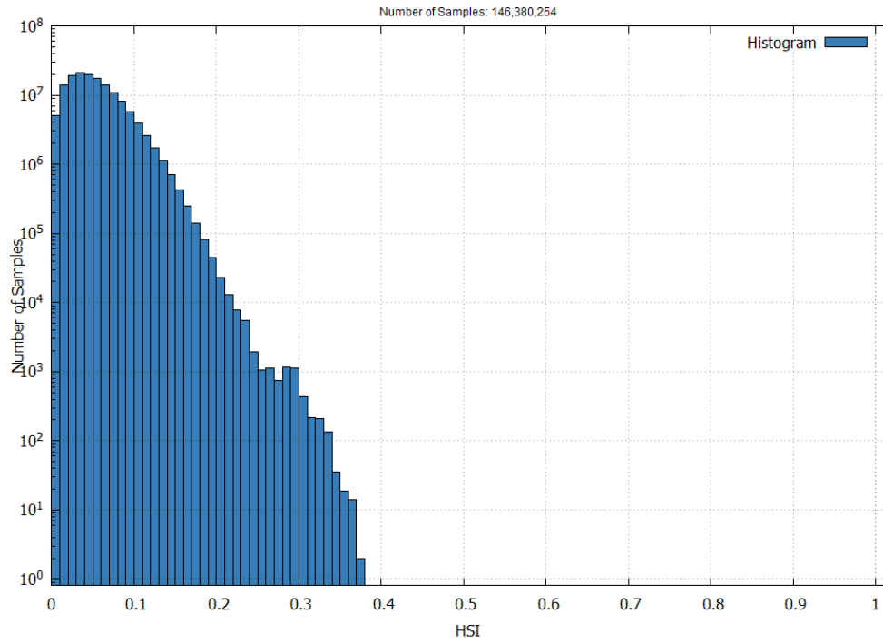
Figure 13 – EGNOS APV-I Horizontal Safety Index in August 2025
