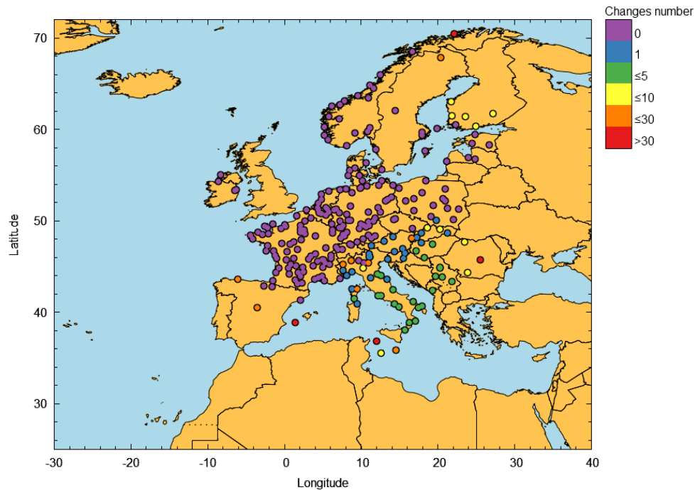
Figure 28 – EGNOS LPV-200 outages in August 2025
