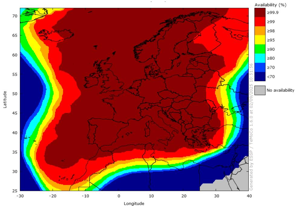
Figure 10 – EGNOS APV-I Availability in August 2025
