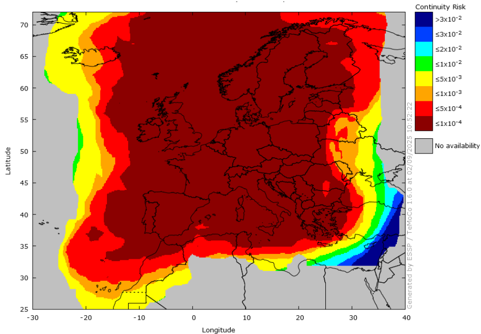
Figure 21 – EGNOS LPV-200 Continuity 3 in August 2025
