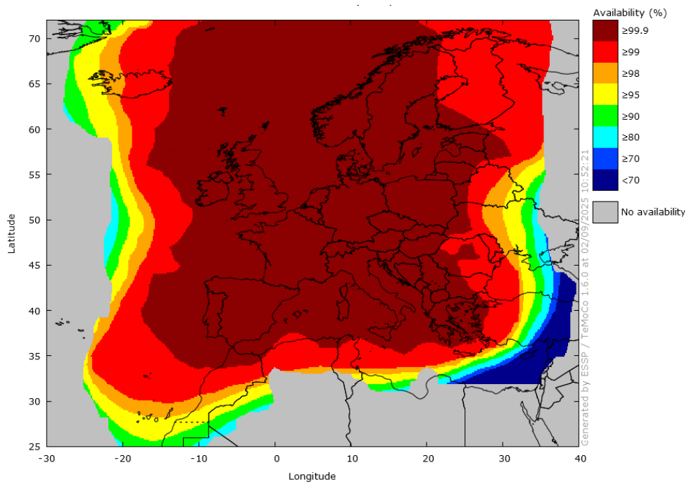
Figure 19 – EGNOS LPV-200 Availability in August 2025
