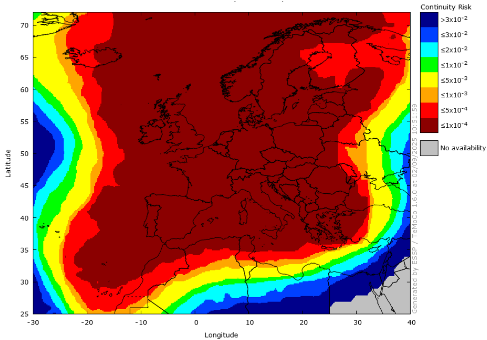
Figure 12 – EGNOS APV-I Continuity in August 2025
