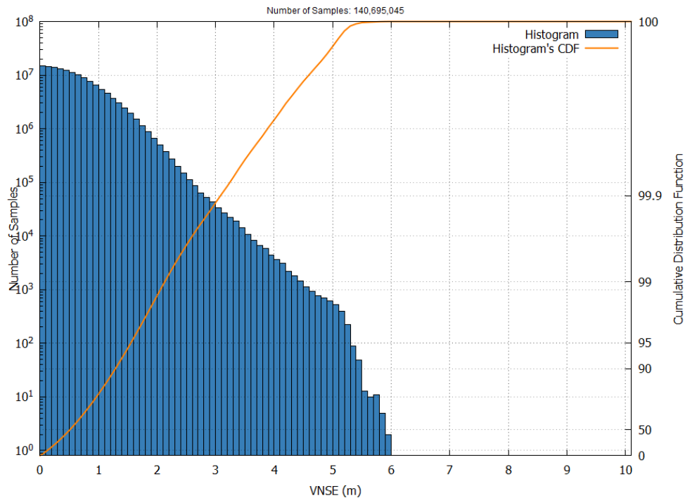
Figure 25 – EGNOS LPV-200 VNSE Histogram and Cumulative Probability in August 2025
