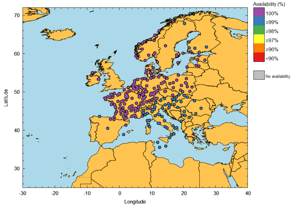
Figure 27 – EGNOS LPV-200 Availability at airports in August 2025
