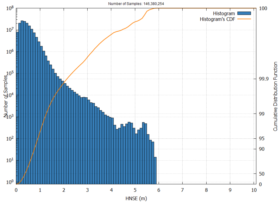
Figure 15 – EGNOS APV-I HNSE Histogram and Cumulative Probability in August 2025
