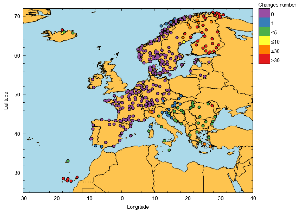
Figure 18 – EGNOS APV-I outages in August 2025
