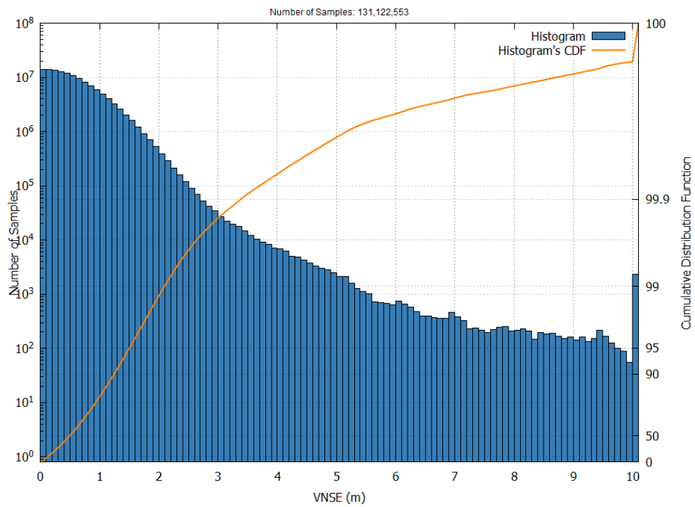
Figure 4 – EGNOS Open Service VNSE Histogram and Cumulative Probability in August 2025
