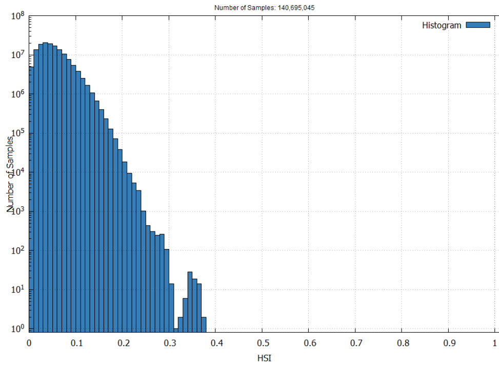
Figure 22 – EGNOS LPV-200 Horizontal Safety Index in August 2025
