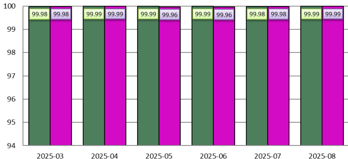
Figure 2 – Trend of EGNOS SIS Availability per GEO for the past 6 months (in green PRN 136; in purple PRN 123)
