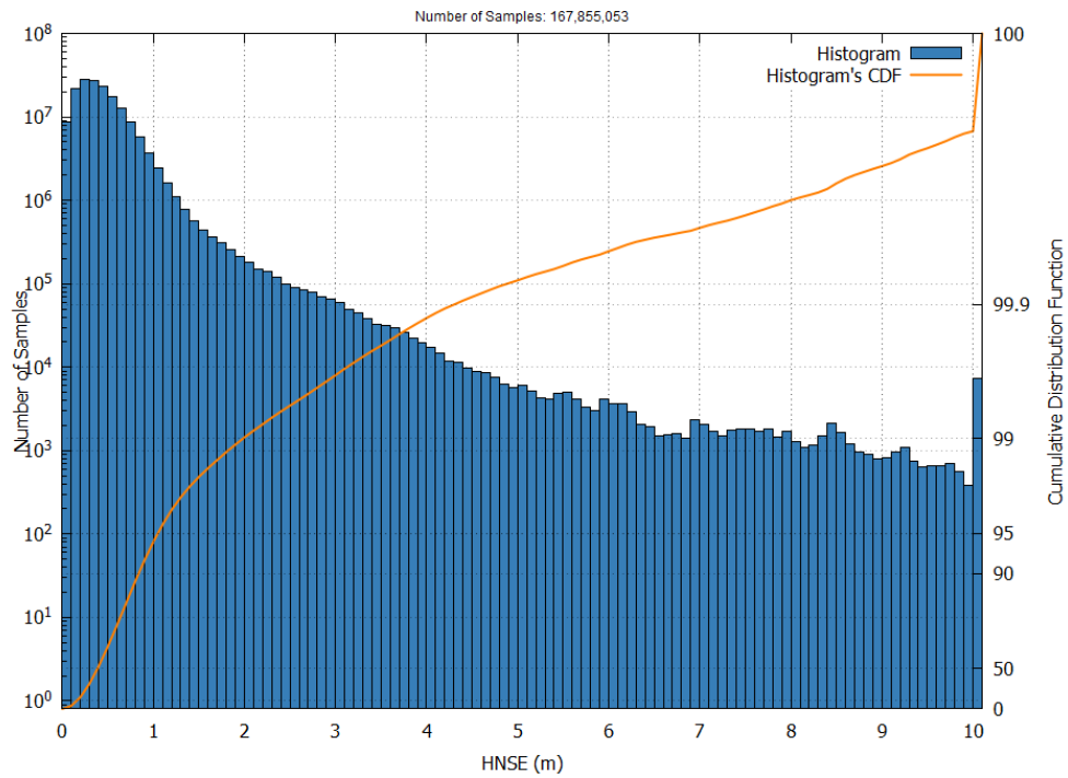
Figure 9 – EGNOS NPA HNSE Histogram and Cumulative Probability in August 2025
