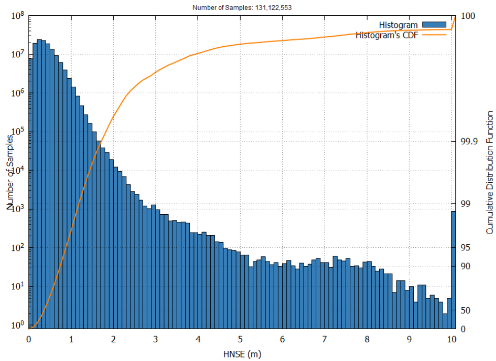
Figure 3 – EGNOS Open Service HNSE Histogram and Cumulative Probability in August 2025
