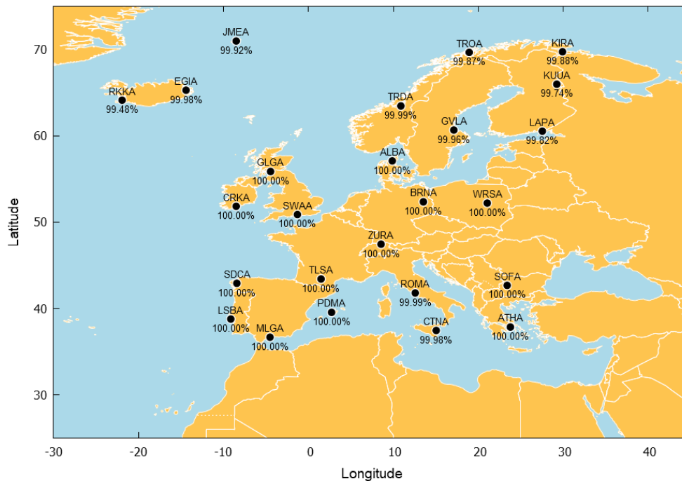
Figure 5 – EGNOS Open Service Availability at reference stations in August 2025
