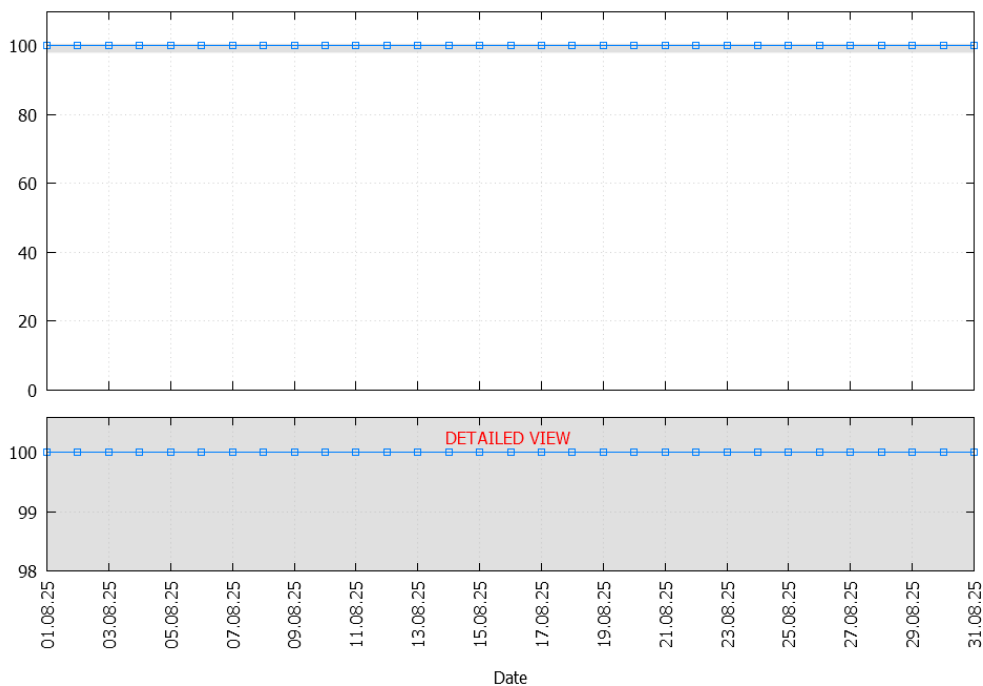
Figure 29 – EGNOS Time Service Availability in August 2025
