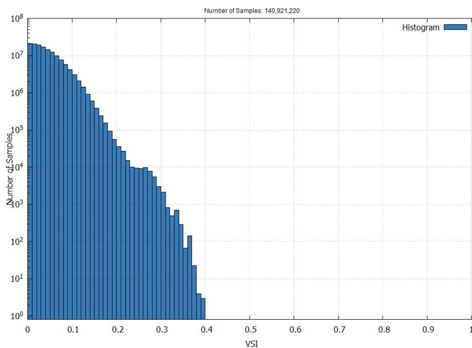
Figure 14 – EGNOS APV-I Vertical Safety Index in June 2025
