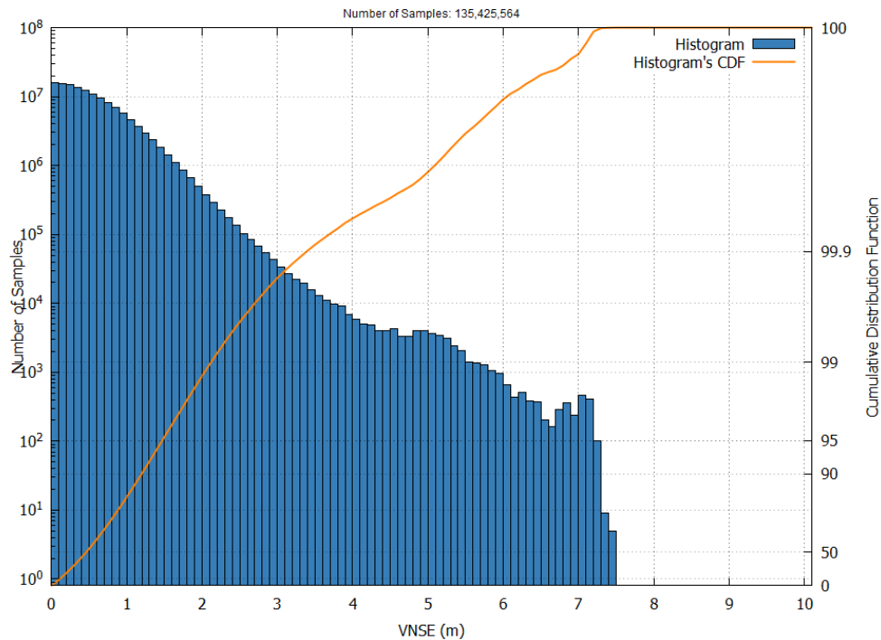
Figure 25 – EGNOS LPV-200 VNSE Histogram and Cumulative Probability in June 2025
