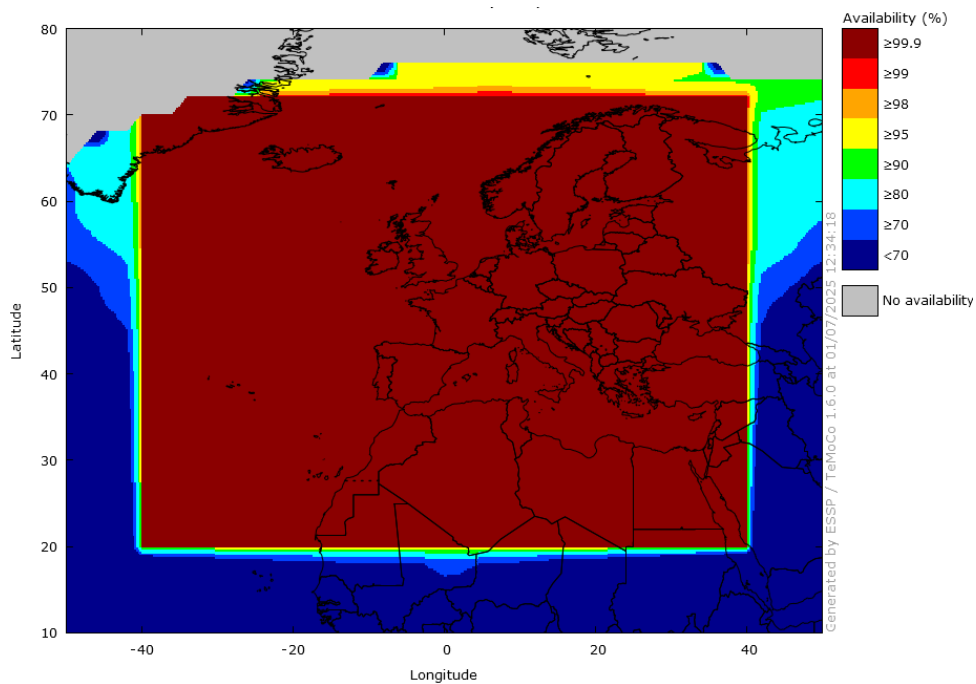
Figure 6 – EGNOS NPA Availability in June 2025
