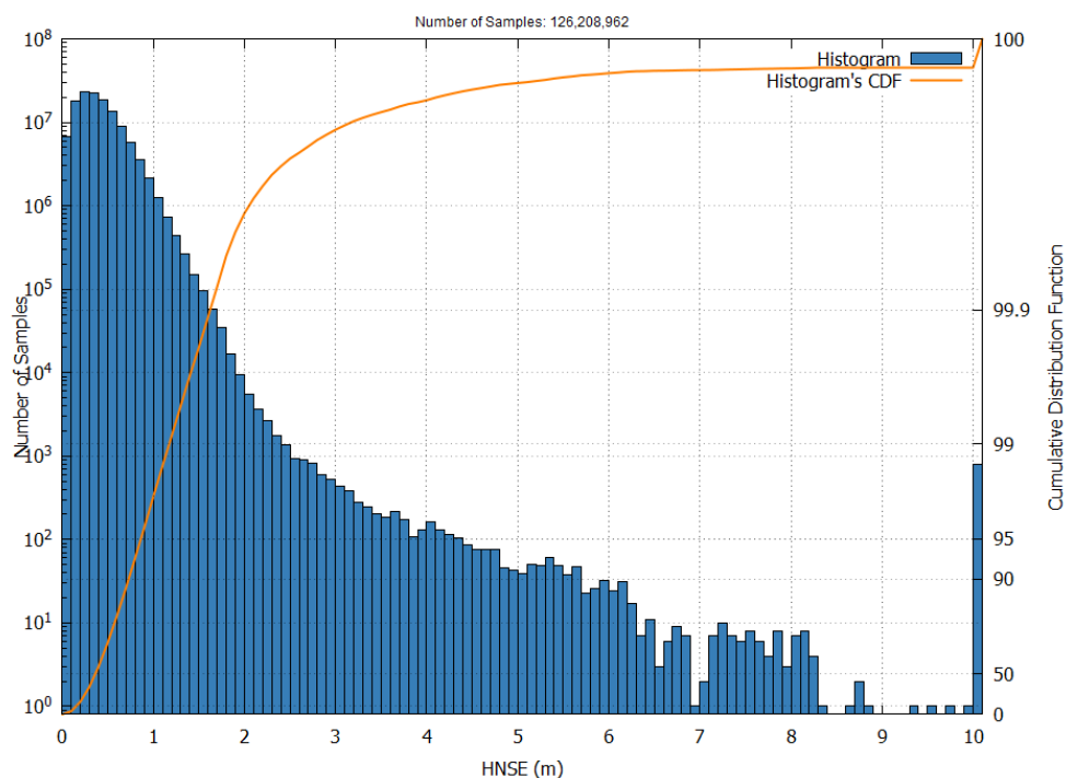
Figure 3 – EGNOS Open Service HNSE Histogram and Cumulative Probability in June 2025
