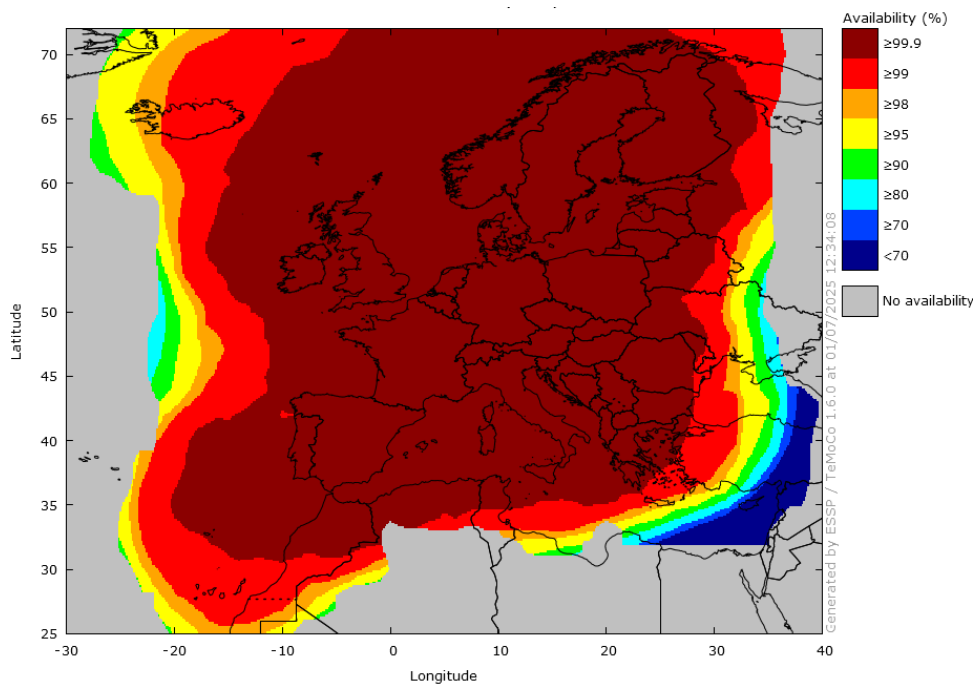
Figure 19 – EGNOS LPV-200 Availability in June 2025
