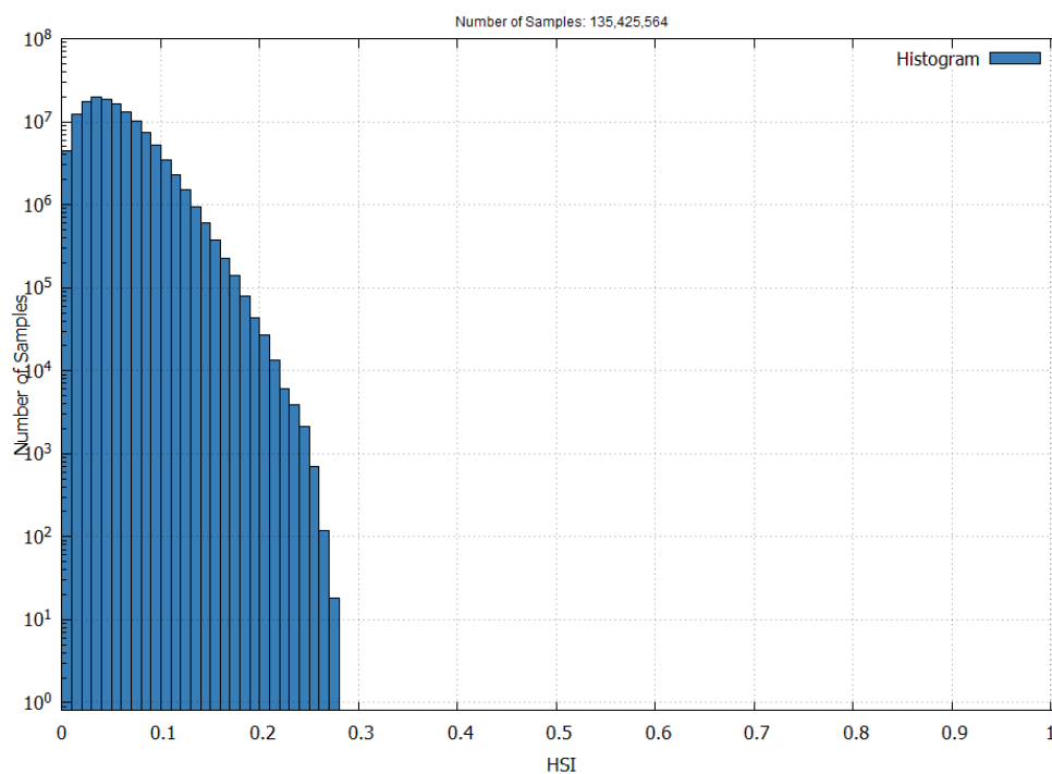
Figure 22 – EGNOS LPV-200 Horizontal Safety Index in June 2025
