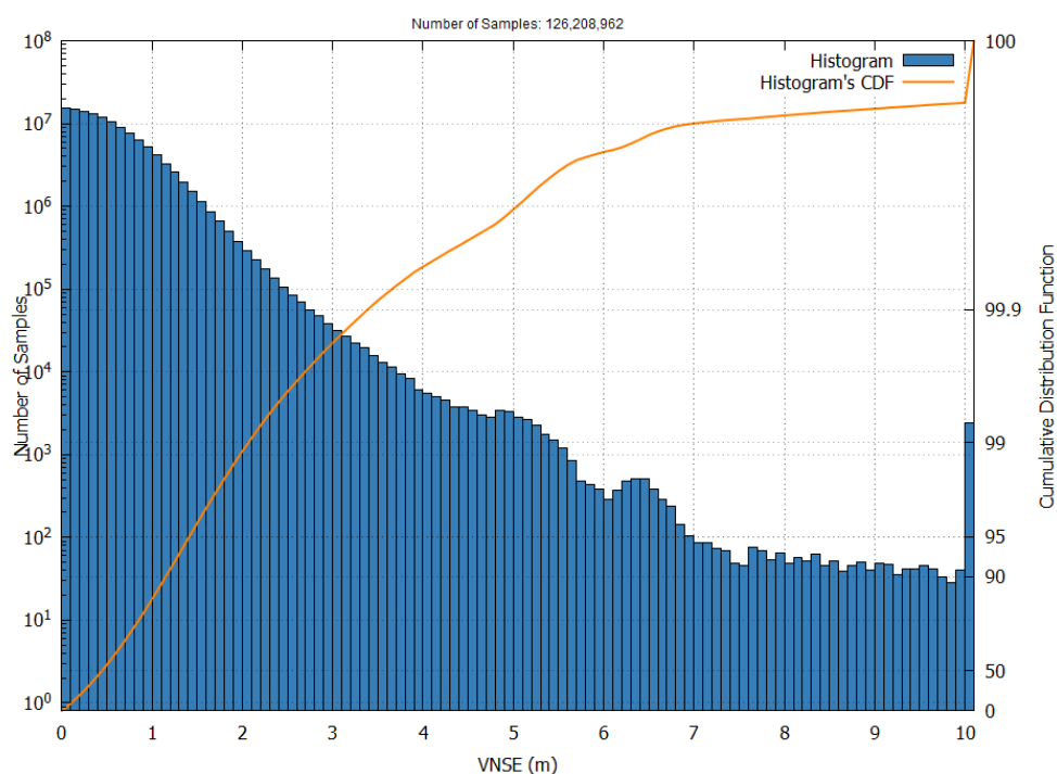
Figure 4 – EGNOS Open Service VNSE Histogram and Cumulative Probability in June 2025
