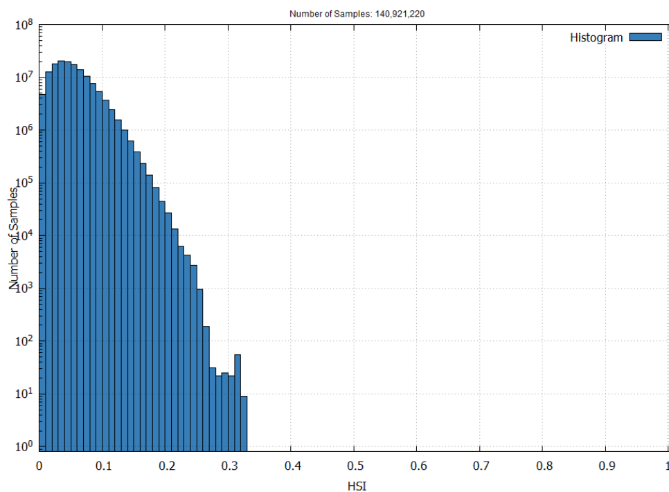
Figure 13 – EGNOS APV-I Horizontal Safety Index in June 2025
