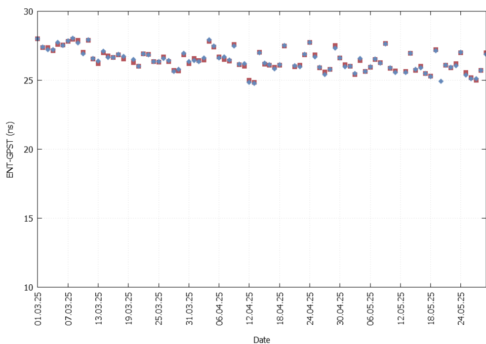
Figure 30 – ENT-GPS offset evolution from March to May 2025 (red PRN 123; blue PRN 136)
