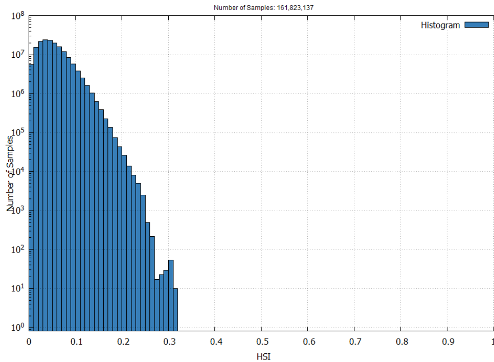
Figure 8 – EGNOS NPA Horizontal Safety Index in June 2025
