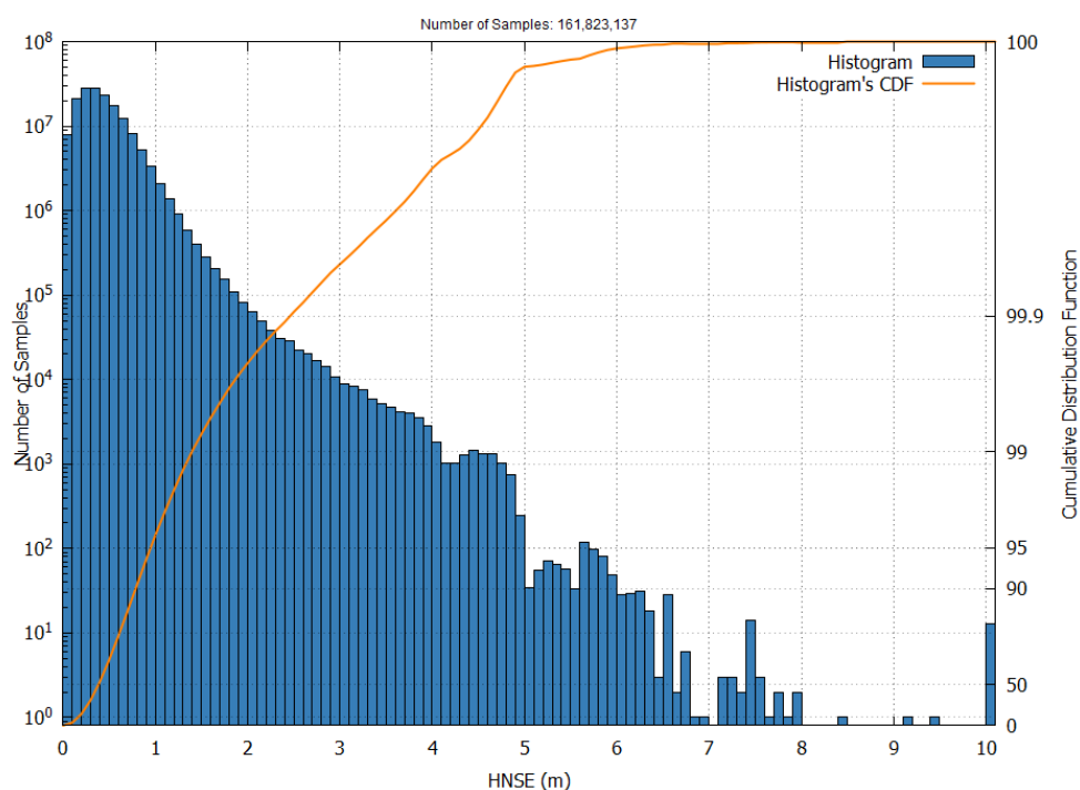
Figure 9 – EGNOS NPA HNSE Histogram and Cumulative Probability in June 2025
