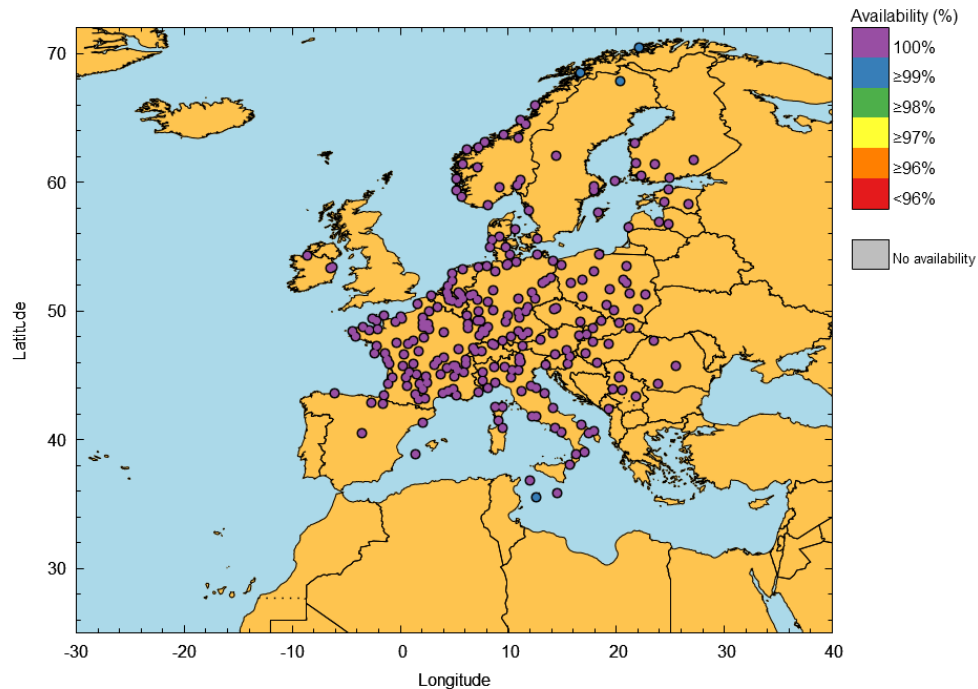
Figure 27 – EGNOS LPV-200 Availability at airports in June 2025
