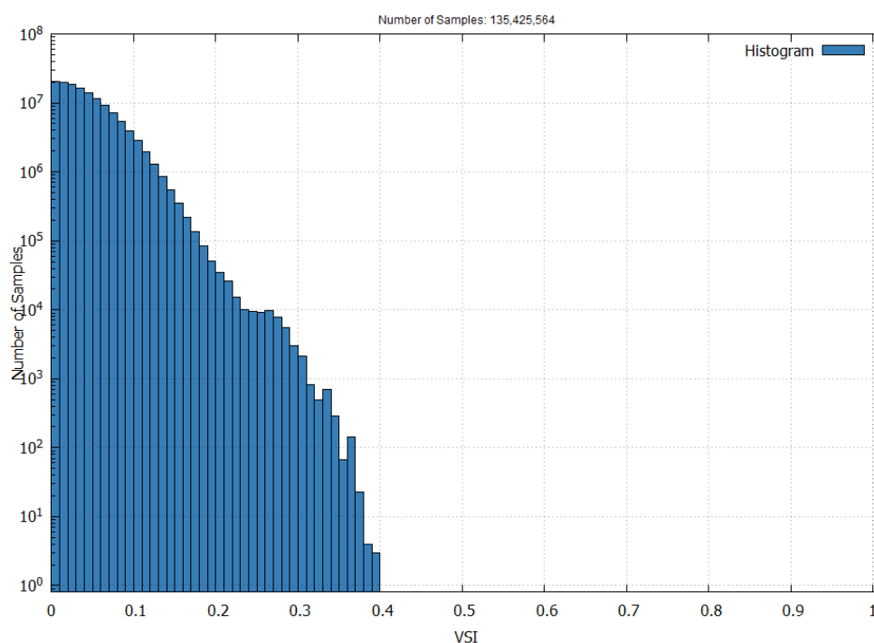
Figure 23 – EGNOS LPV-200 Vertical Safety Index in June 2025
