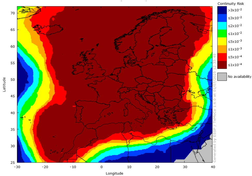
Figure 12 – EGNOS APV-I Continuity in June 2025
