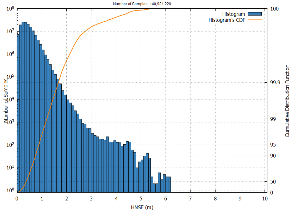
Figure 15 – EGNOS APV-I HNSE Histogram and Cumulative Probability in June 2025
