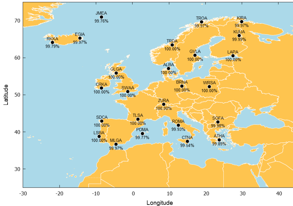
Figure 5 – EGNOS Open Service Availability at reference stations in June 2025
