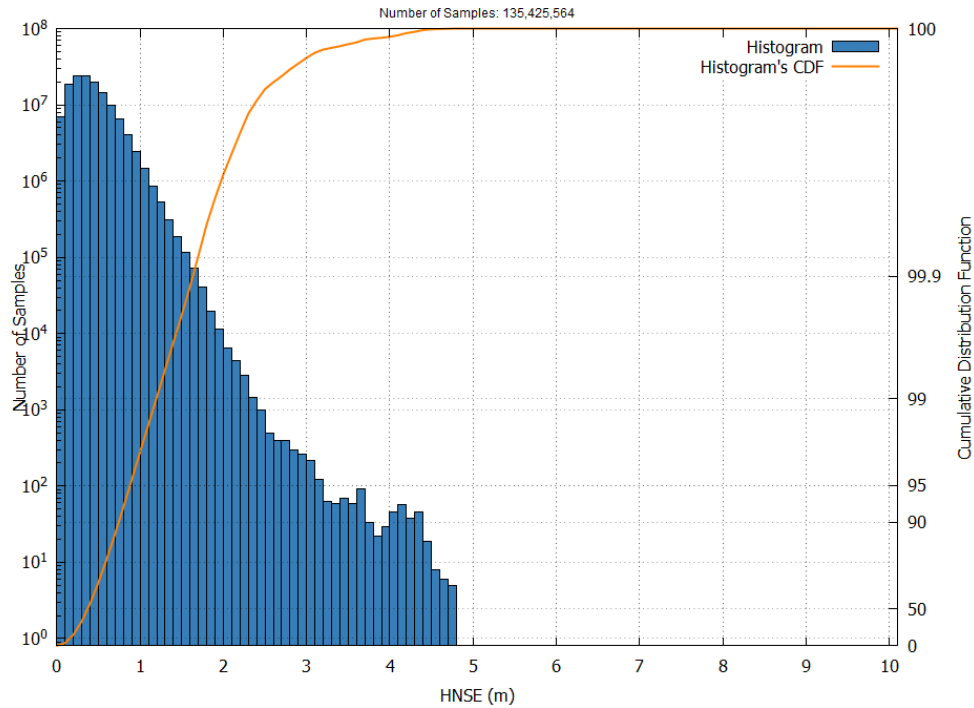
Figure 24 – EGNOS LPV-200 HNSE Histogram and Cumulative Probability in June 2025
