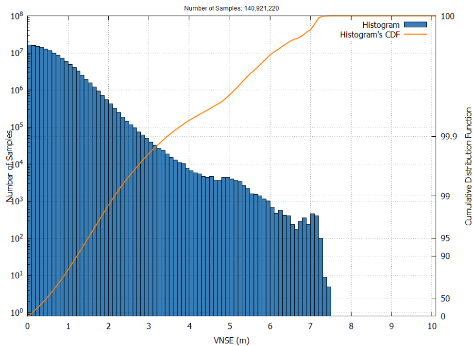
Figure 16 – EGNOS APV-I VNSE Histogram and Cumulative Probability in June 2025
