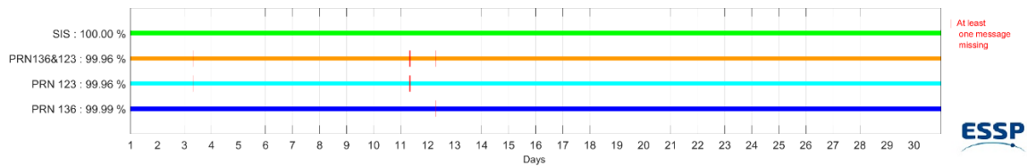
Figure 1 - EGNOS SIS & PRN Availability for June 2025
