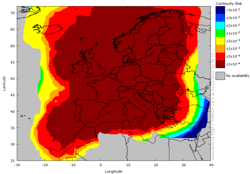
Figure 21 – EGNOS LPV-200 Continuity 2 in June 2025
