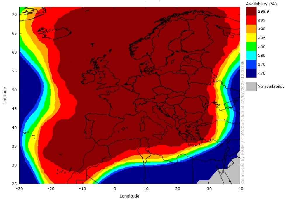
Figure 10 – EGNOS APV-I Availability in June 2025
