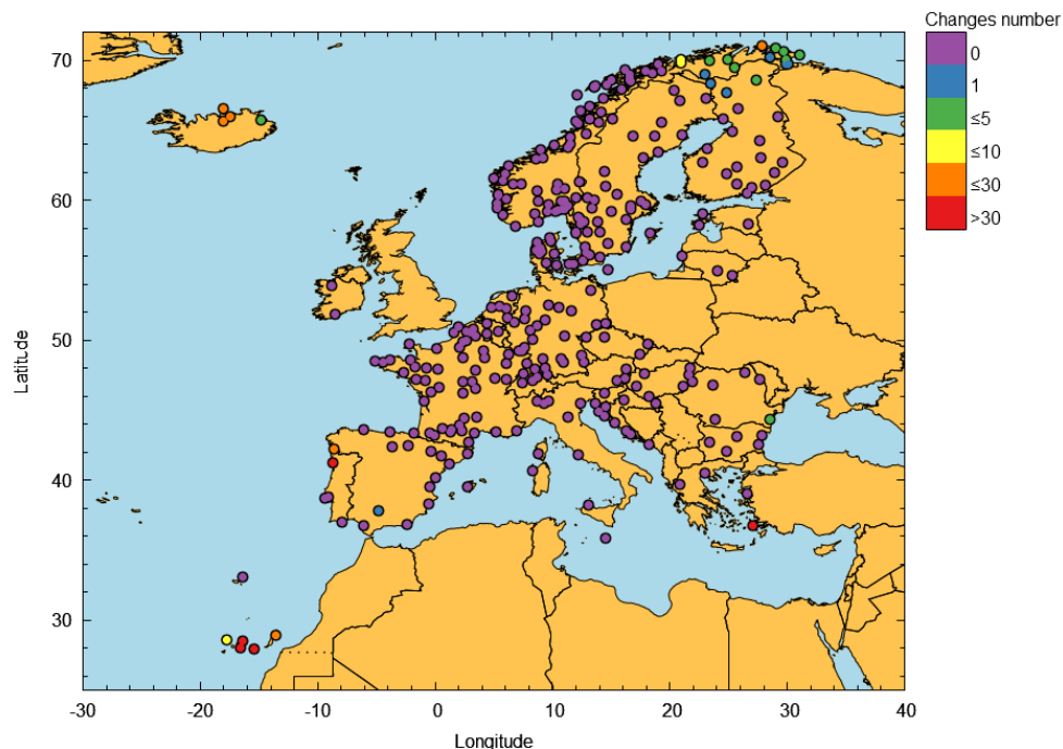
Figure 18 – EGNOS APV-I outages in June 2025
