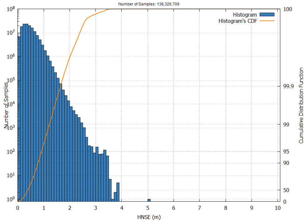
Figure 24 – EGNOS LPV-200 HNSE Histogram and Cumulative Probability in May 2025
