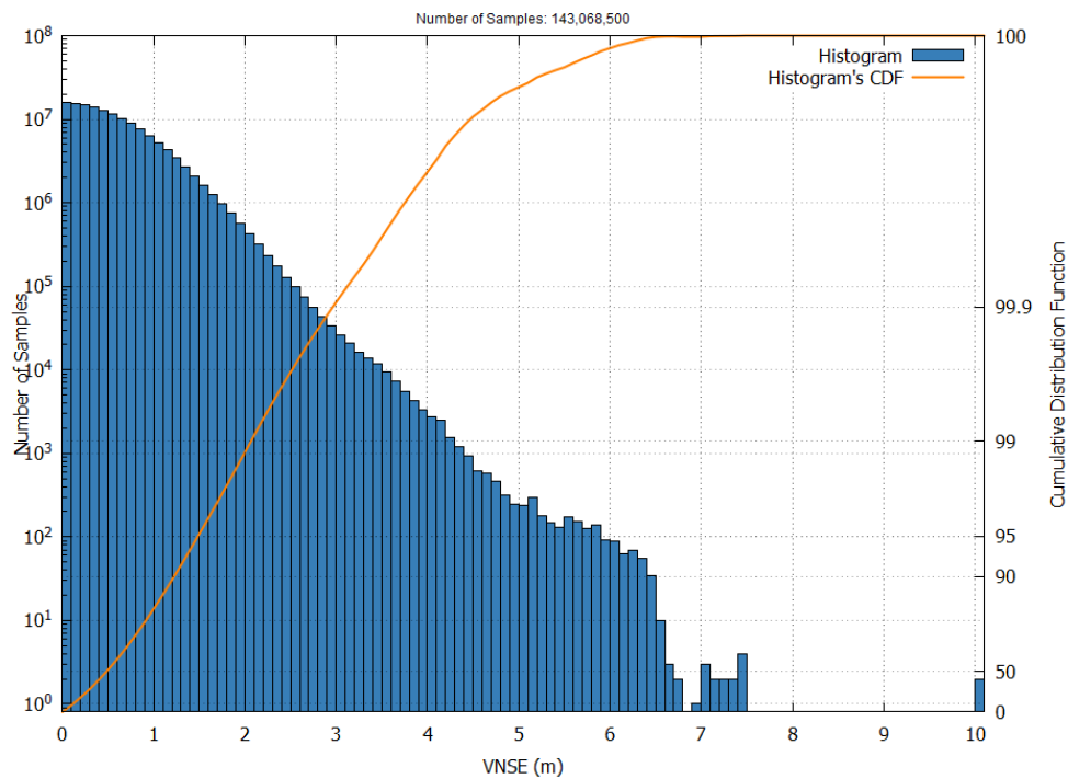
Figure 16 – EGNOS APV-I VNSE Histogram and Cumulative Probability in May 2025
