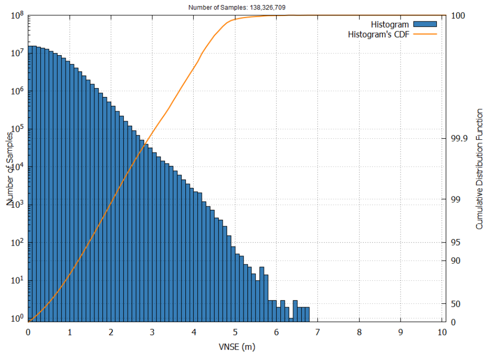
Figure 25 – EGNOS LPV-200 VNSE Histogram and Cumulative Probability in May 2025
