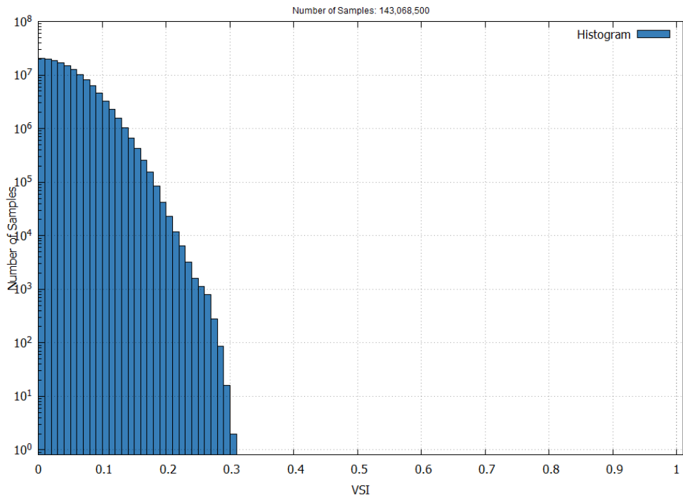
Figure 14 – EGNOS APV-I Vertical Safety Index in May 2025
