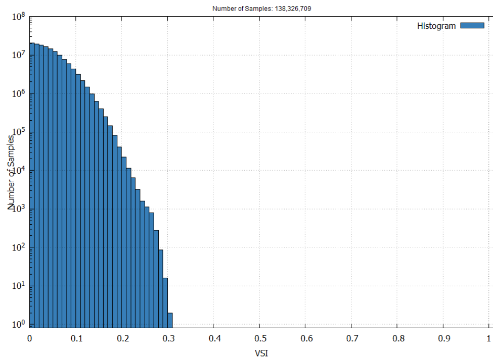
Figure 23 – EGNOS LPV-200 Vertical Safety Index in May 2025
