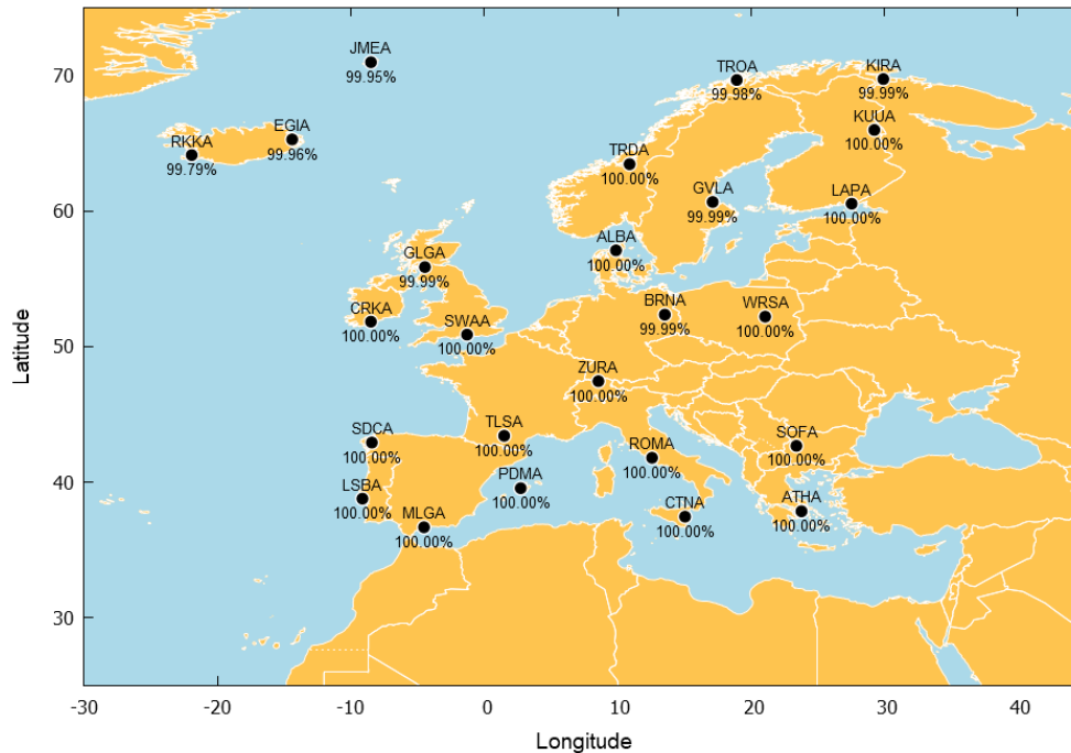
Figure 5 – EGNOS Open Service Availability at reference stations in May 2025
