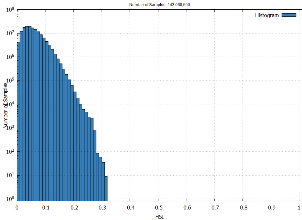
Figure 13 – EGNOS APV-I Horizontal Safety Index in May 2025
