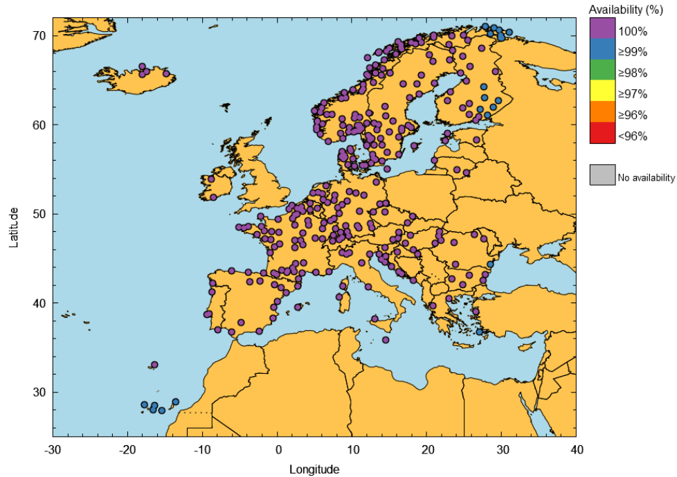
Figure 17 – EGNOS APV-I Availability at airports in May 2025
