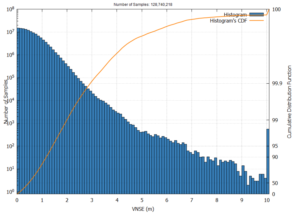
Figure 4 – EGNOS Open Service VNSE Histogram and Cumulative Probability in May 2025
