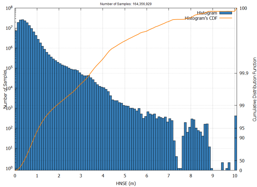
Figure 9 – EGNOS NPA HNSE Histogram and Cumulative Probability in May 2025
