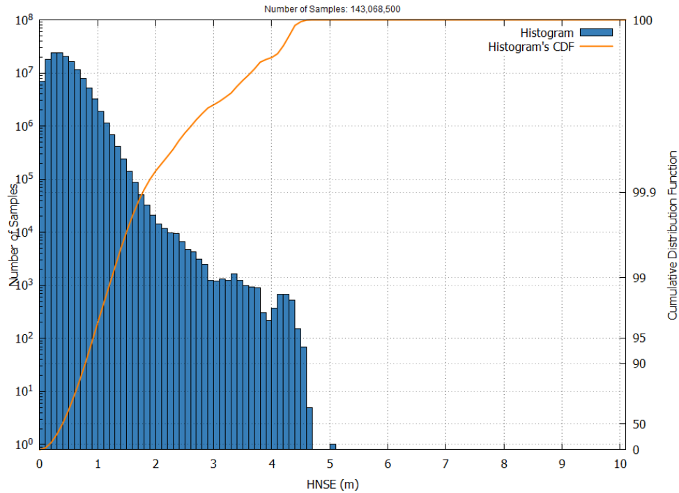
Figure 15 – EGNOS APV-I HNSE Histogram and Cumulative Probability in May 2025
