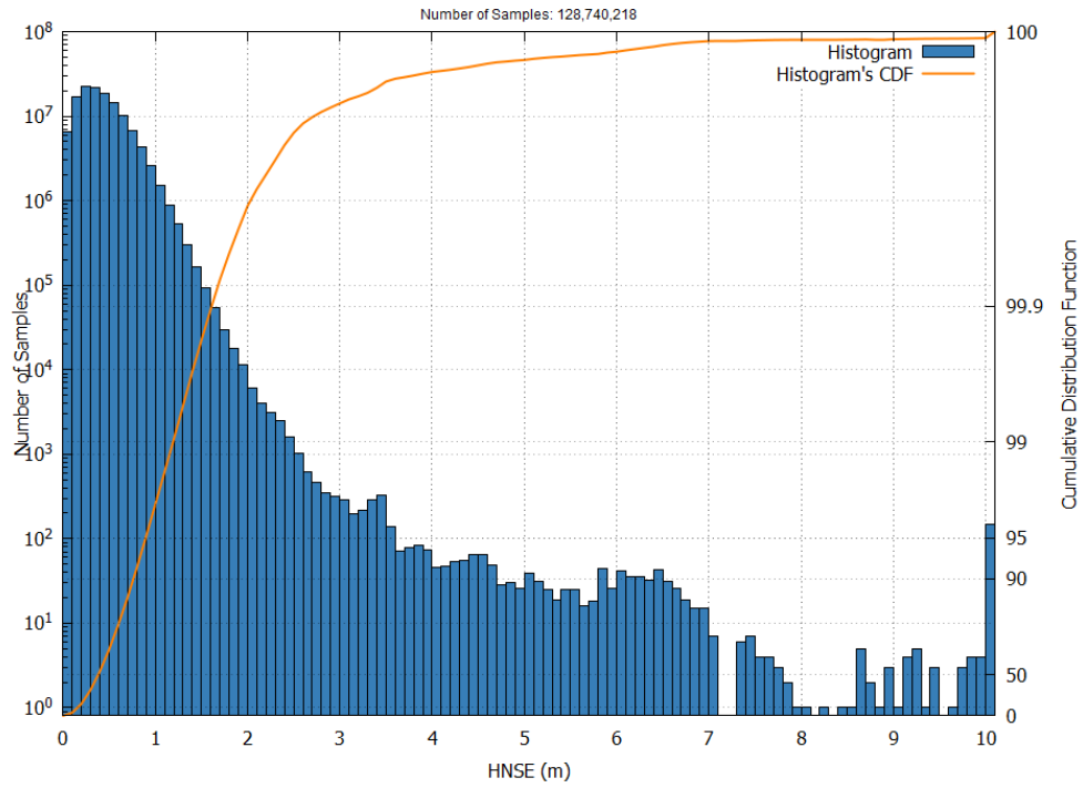
Figure 3 – EGNOS Open Service HNSE Histogram and Cumulative Probability in May 2025
