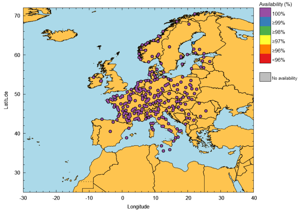
Figure 27 – EGNOS LPV-200 Availability at airports in May 2025
