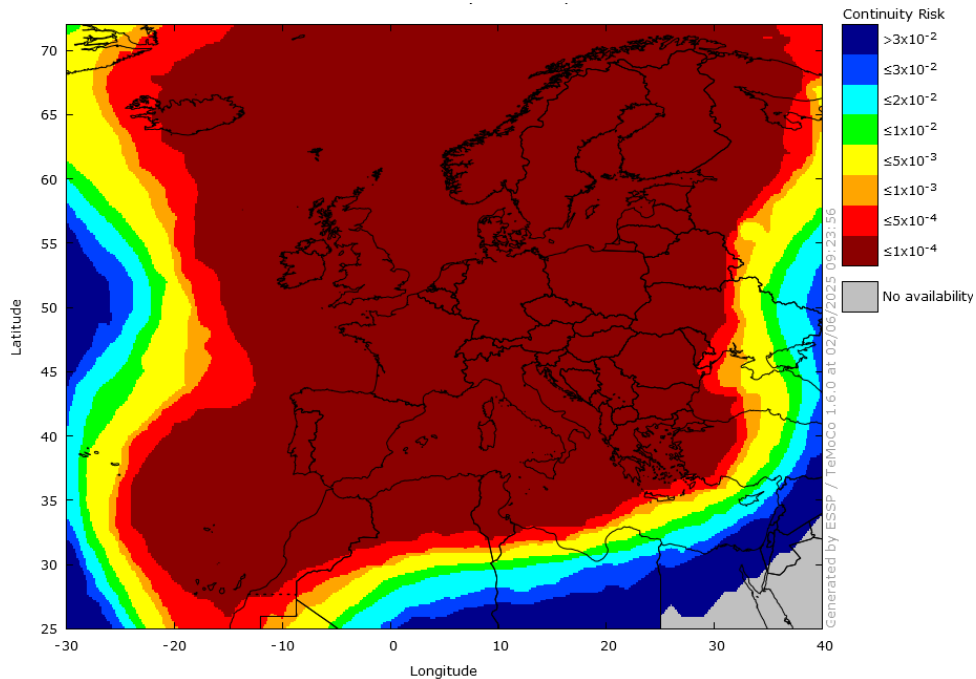
Figure 12 – EGNOS APV-I Continuity in May 2025
