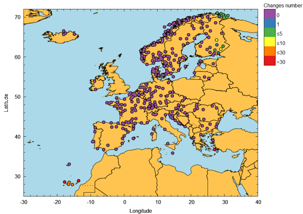
Figure 18 – EGNOS APV-I outages in May 2025
