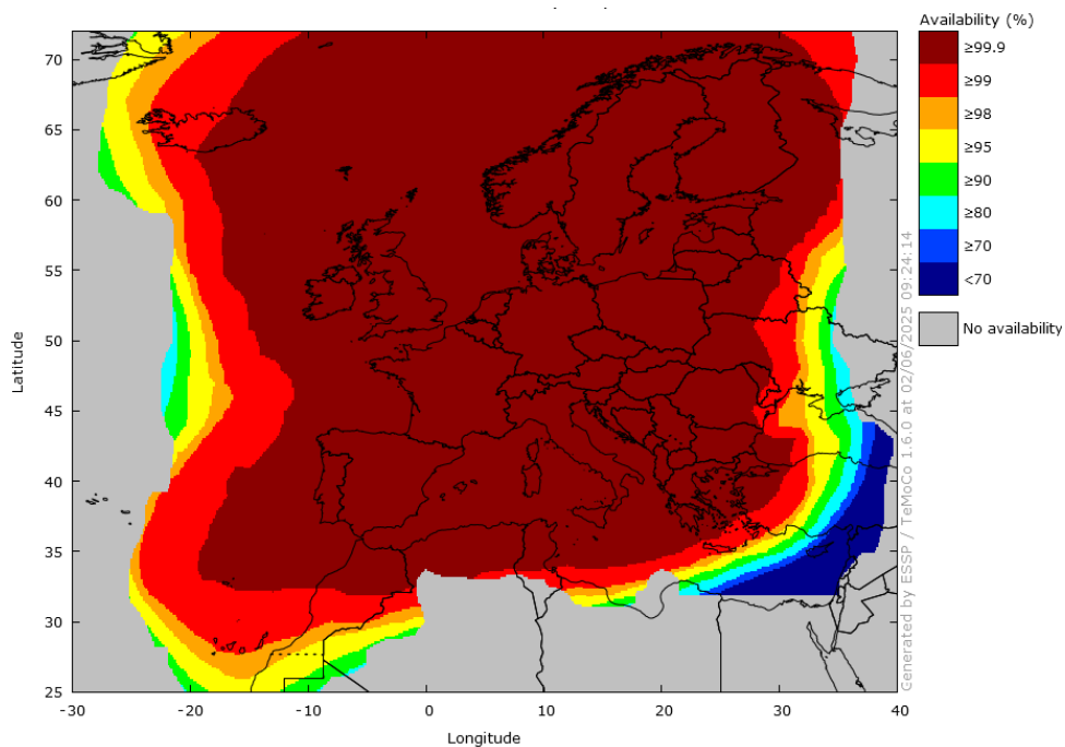
Figure 19 – EGNOS LPV-200 Availability in May 2025
