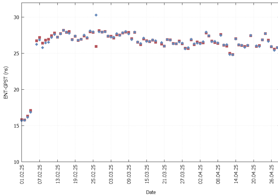
Figure 30 – ENT-GPS offset evolution from February to April 2025 (red PRN 123; blue PRN 136)
