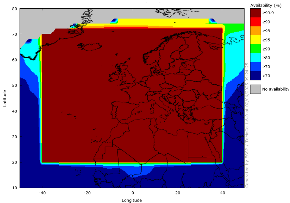
Figure 6 – EGNOS NPA Availability in May 2025
