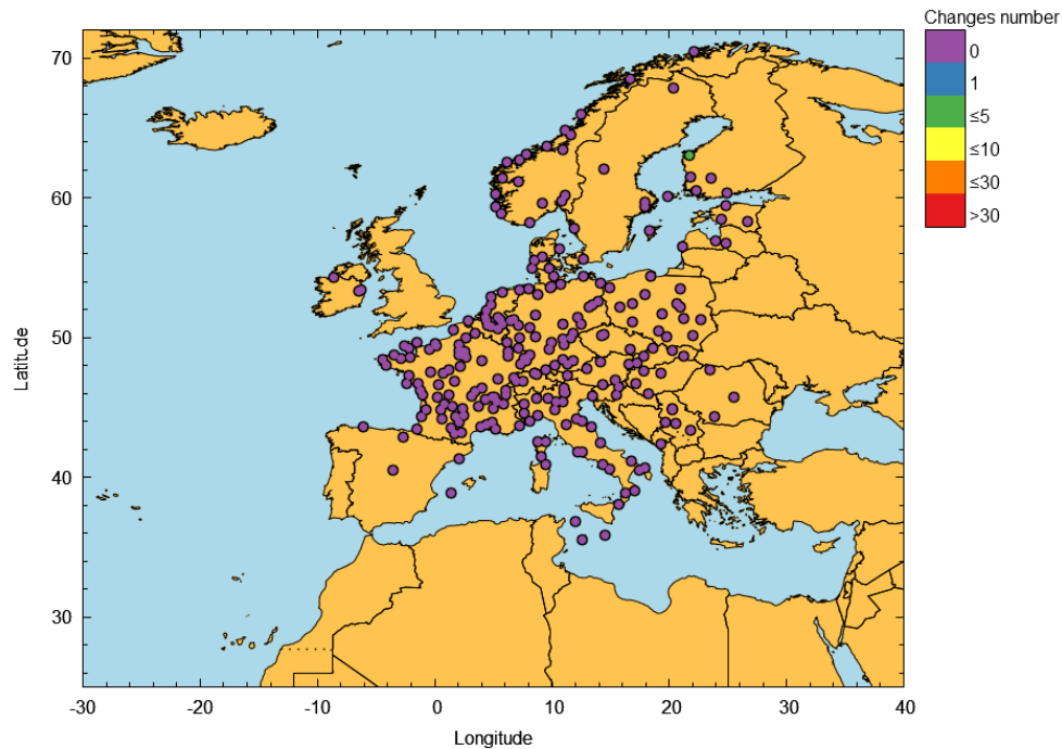
Figure 28 – EGNOS LPV-200 outages in May 2025
