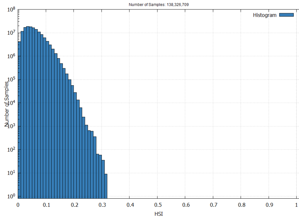
Figure 22 – EGNOS LPV-200 Horizontal Safety Index in May 2025
