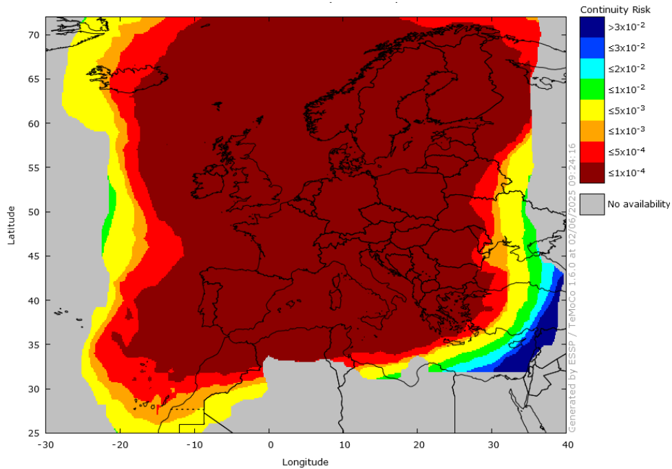
Figure 21 – EGNOS LPV-200 Continuity 2 in May 2025
