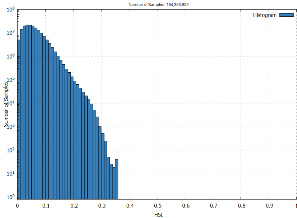
Figure 8 – EGNOS NPA Horizontal Safety Index in May 2025
