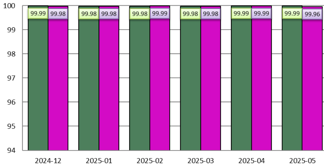
Figure 2 – Trend of EGNOS SIS Availability per GEO for the past 6 months (in green PRN 136; in purple PRN 123)
