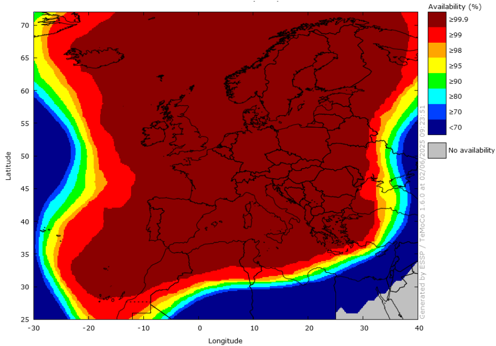
Figure 10 – EGNOS APV-I Availability in May 2025
