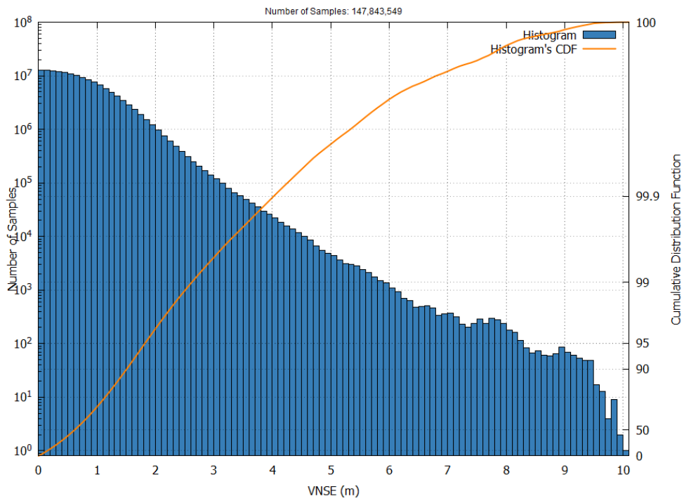
Figure 16 – EGNOS APV-I VNSE Histogram and Cumulative Probability in December 2024
