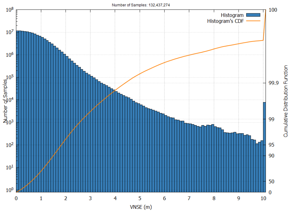
Figure 4 – EGNOS Open Service VNSE Histogram and Cumulative Probability in December 2024
