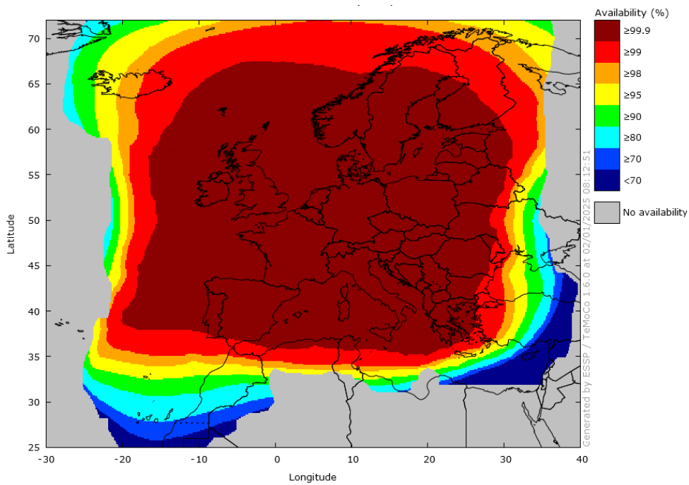
Figure 19 – EGNOS LPV-200 Availability in December 2024
