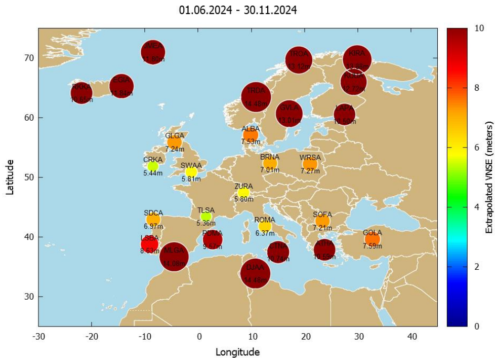
Figure 28 - Extrapolated VNSE at 10-7/150s in the RIMS within the LPV200 commitment
