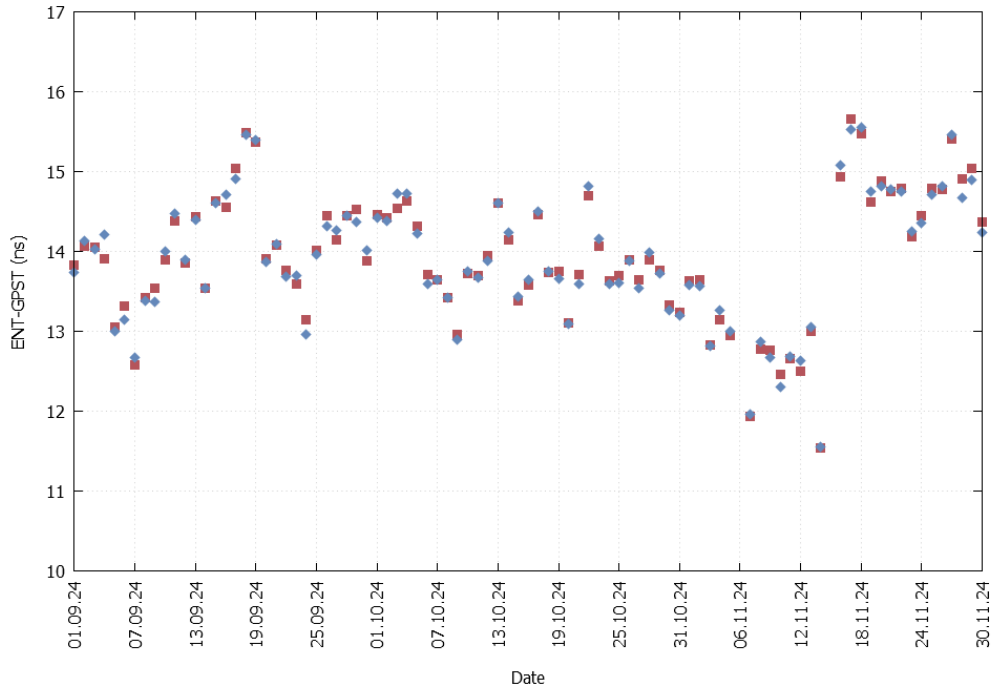
Figure 30 – ENT-GPS offset evolution from September to November 2024 (red PRN 123; blue PRN 136)
