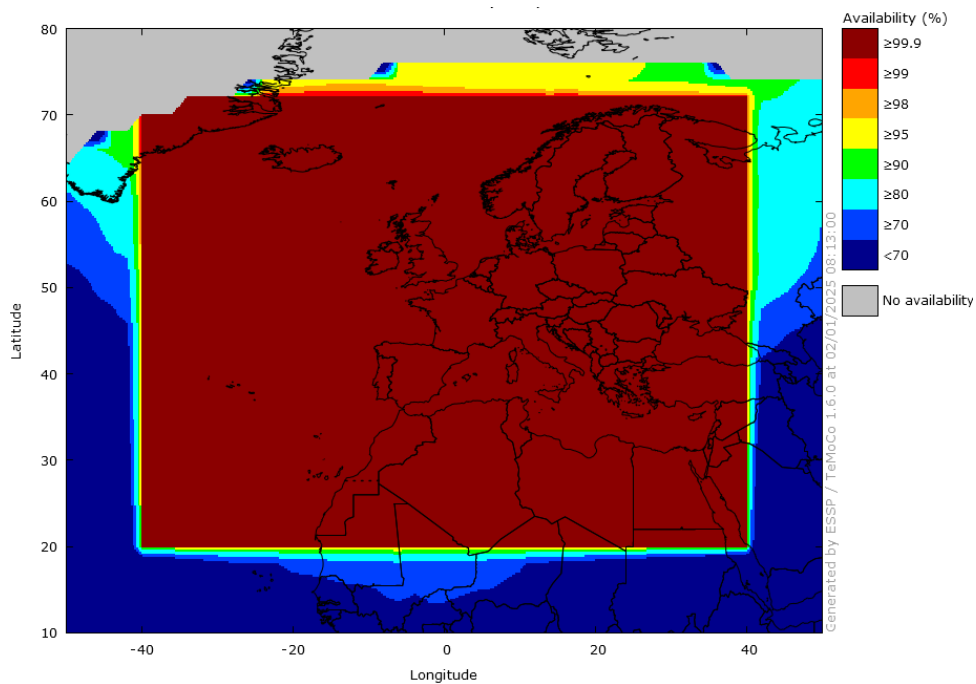
Figure 6 – EGNOS NPA Availability in December 2024
