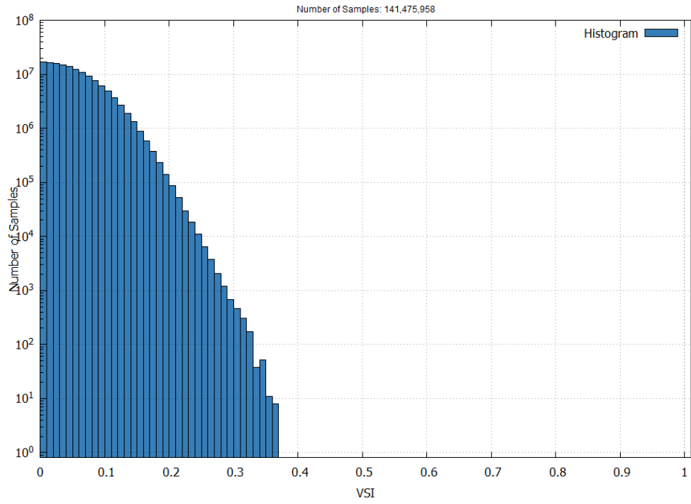
Figure 23 – EGNOS LPV-200 Vertical Safety Index in December 2024
