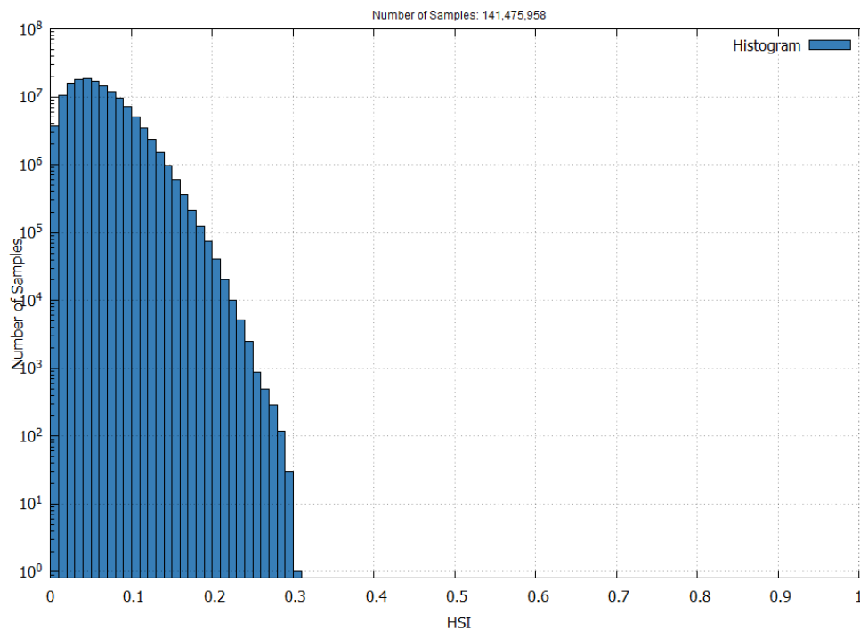
Figure 22 – EGNOS LPV-200 Horizontal Safety Index in December 2024
