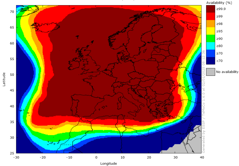
Figure 10 – EGNOS APV-I Availability in December 2024
