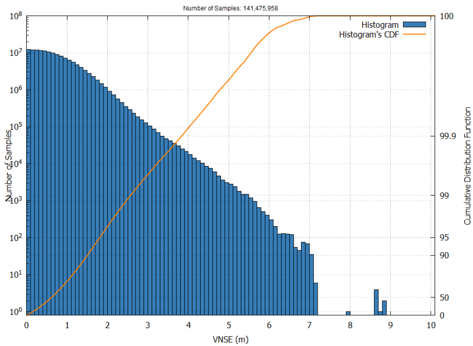
Figure 25 – EGNOS LPV-200 VNSE Histogram and Cumulative Probability in December 2024
