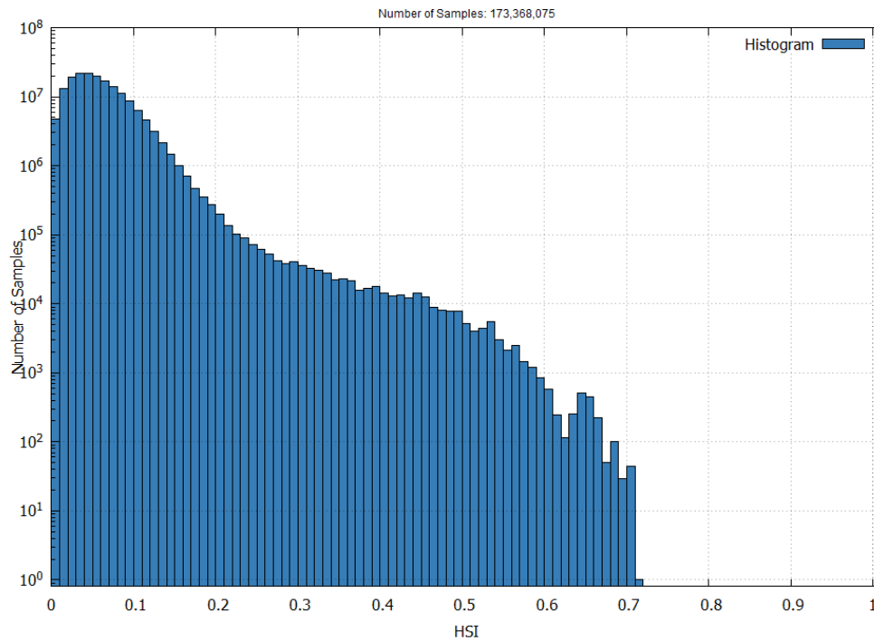
Figure 8 – EGNOS NPA Horizontal Safety Index in December 2024
