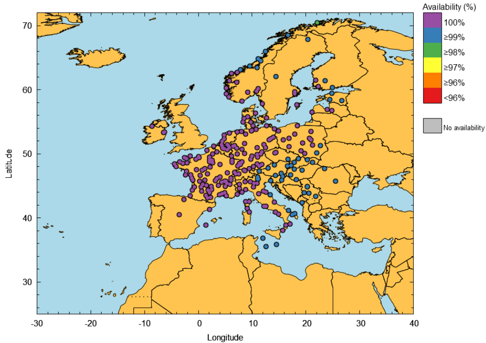
Figure 26 – EGNOS LPV-200 Availability at airports in December 2024
