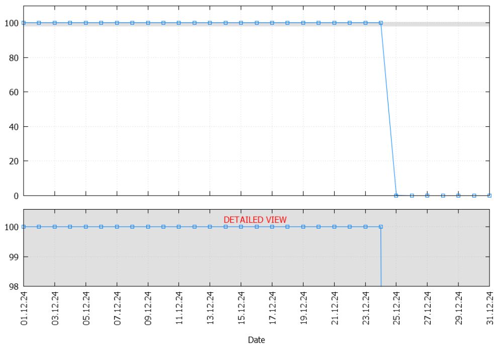
Figure 29 – EGNOS Time Service Availability in December 2024
