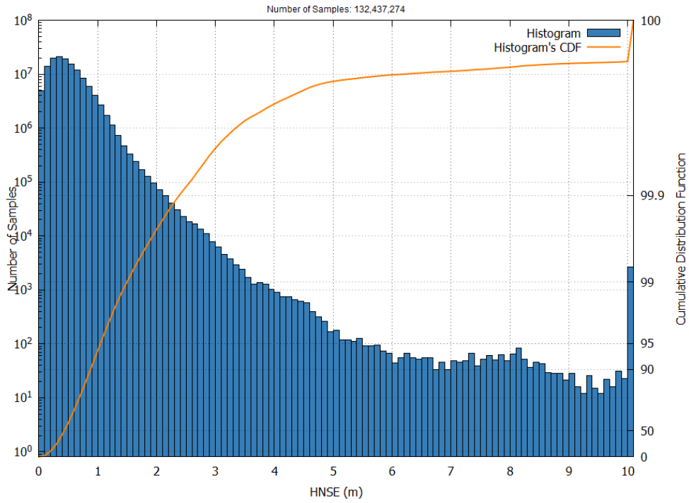
Figure 3 – EGNOS Open Service HNSE Histogram and Cumulative Probability in December 2024
