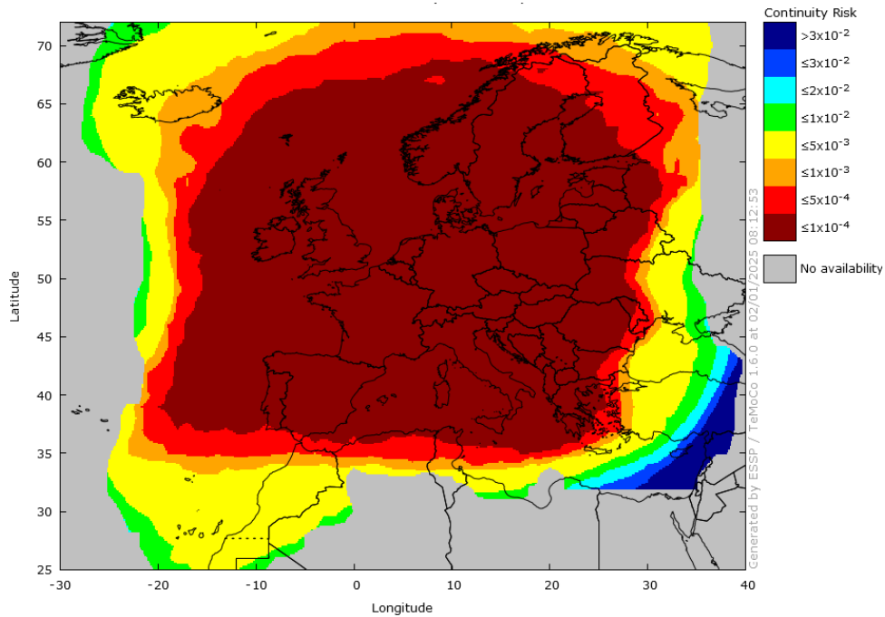
Figure 21 – EGNOS LPV-200 Continuity 3 in December 2024
