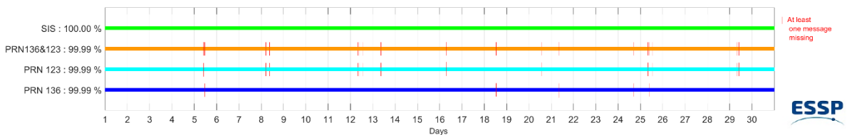
Figure 1 - EGNOS SIS & PRN Availability for December 2024
