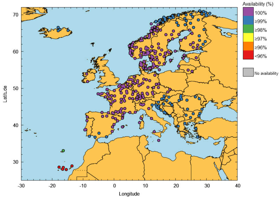
Figure 17 – EGNOS APV-I Availability at airports in December 2024
