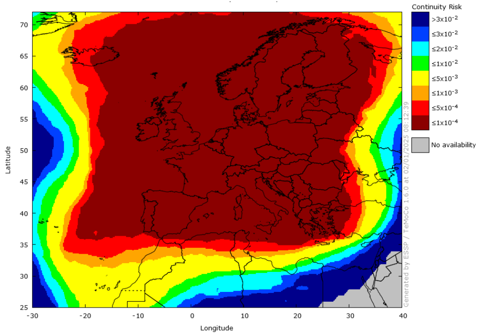
Figure 12 – EGNOS APV-I Continuity in December 2024
