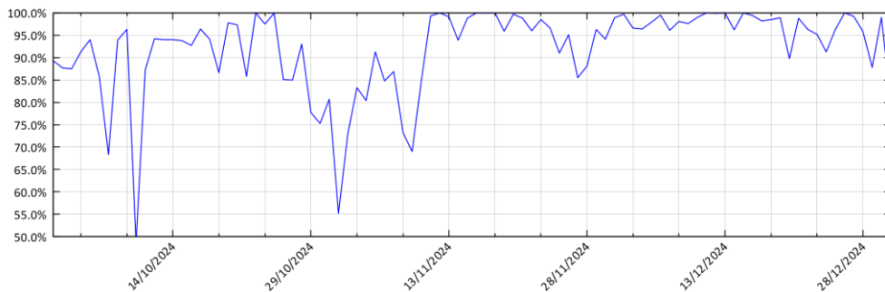
Figure 20 – EGNOS LPV-200 Availability compliance trend for the last 3 months before December 2024
