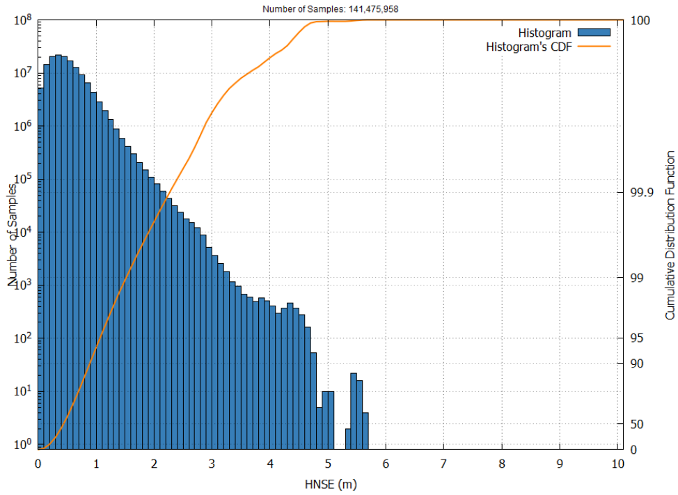
Figure 24 – EGNOS LPV-200 HNSE Histogram and Cumulative Probability in December 2024
