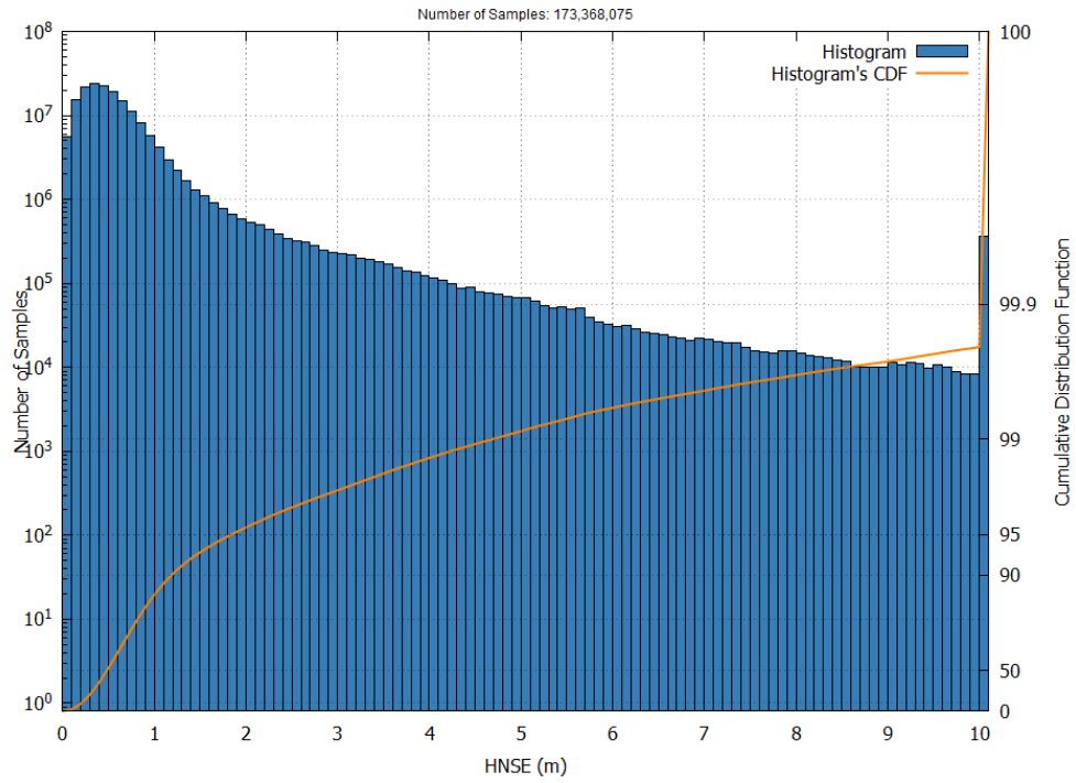
Figure 9 – EGNOS NPA HNSE Histogram and Cumulative Probability in December 2024
