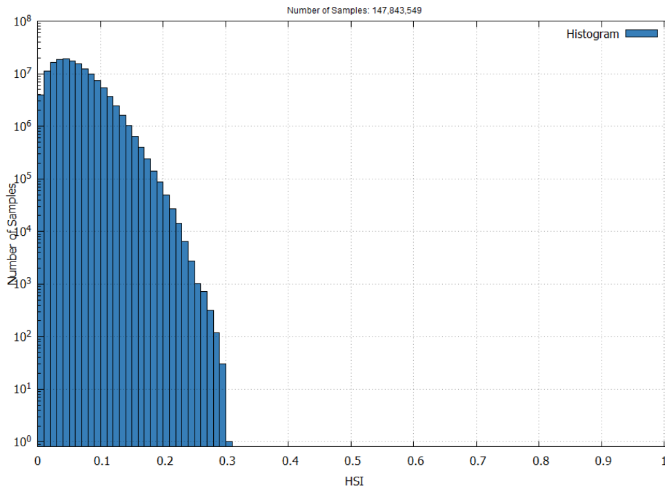
Figure 13 – EGNOS APV-I Horizontal Safety Index in December 2024
