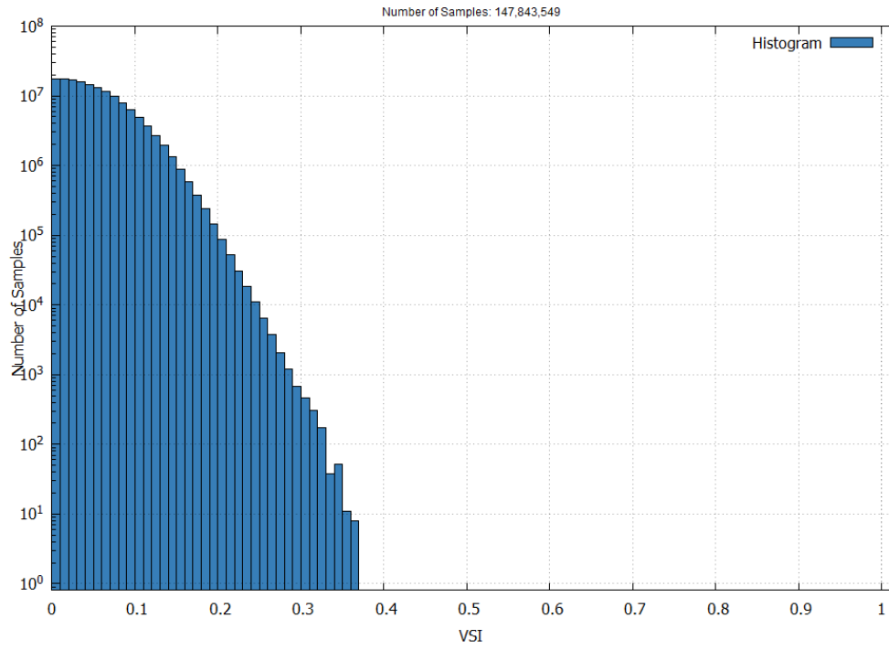
Figure 14 – EGNOS APV-I Vertical Safety Index in December 2024
