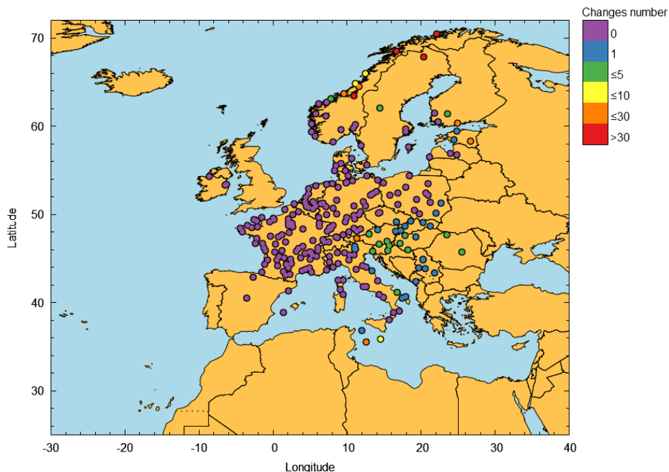
Figure 27 – EGNOS LPV-200 outages in December 2024
