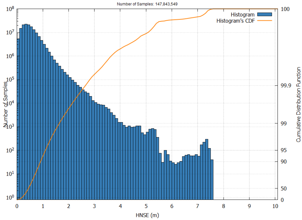
Figure 15 – EGNOS APV-I HNSE Histogram and Cumulative Probability in December 2024
