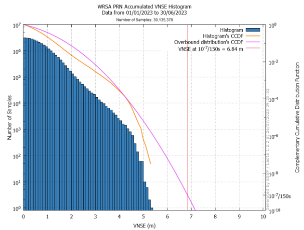
Figure 44: Extrapolated LPV200 VNSE at 10-7/150s in TRO (left) & WRS (right)
