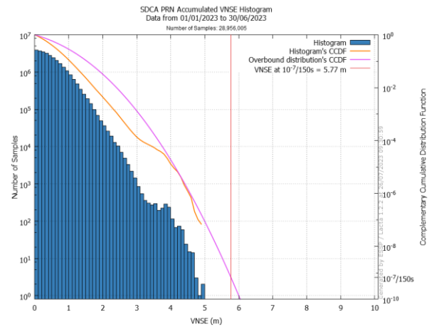
Figure 41: Extrapolated LPV200 VNSE at 10 -7 /150s in ROM (left) & SDC (right)
