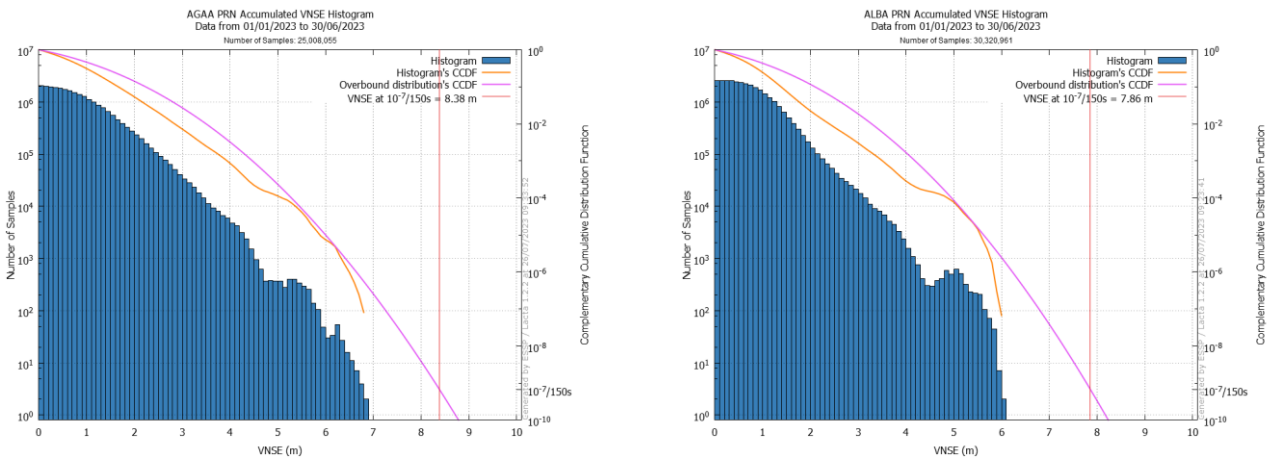
Figure 31: Extrapolated LPV200 VNSE at 10 -7 /150s in AGA (left) & ALB (right)
