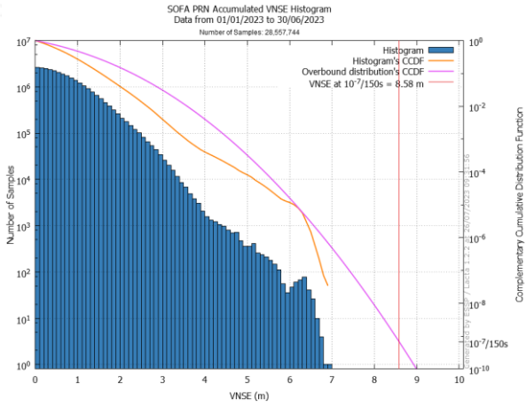
Figure 42: Extrapolated LPV200 VNSE at 10-7/150s in SOF (left) & SWA (right)
