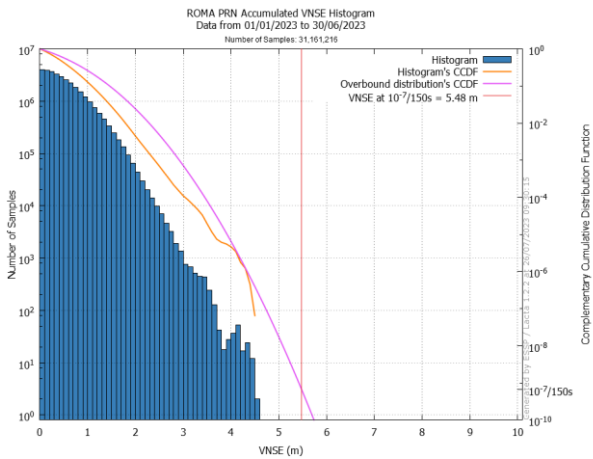
Figure 41: Extrapolated LPV200 VNSE at 10 -7 /150s in ROM (left) & SDC (right)
