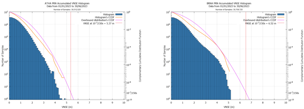
Figure 32: Extrapolated LPV200 VNSE at 10 -7 /150s in ATH (left) & BRN (right)
