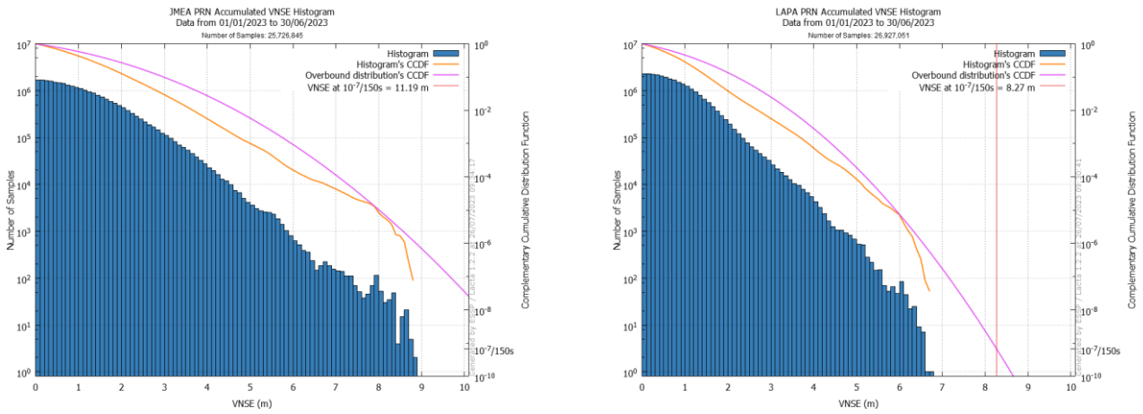
Figure 37: Extrapolated LPV200 VNSE at 10-7/150s in JME (left) & LAP (right)
