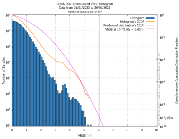
Figure 40: Extrapolated LPV200 VNSE at 10 -7 /150s in PDM (left) & RKK (right)
