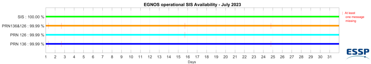
Figure 1 – EGNOS SIS & PRN Availability for July 2023
