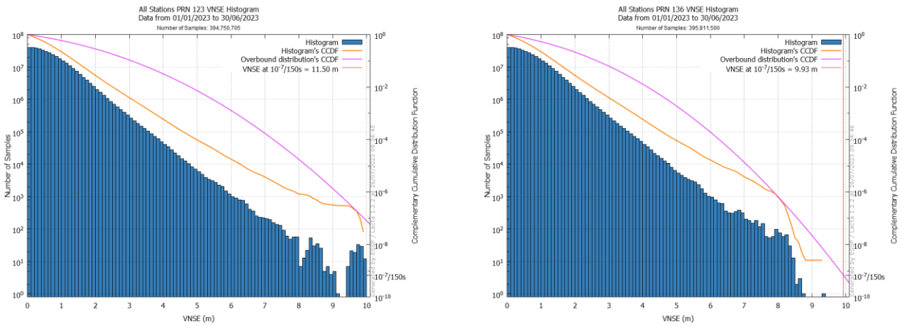
Figure 46: Extrapolated LPV200 VNSE at 10-7/150s - all RIMS - PRN123 (left) & PRN136 (right)
