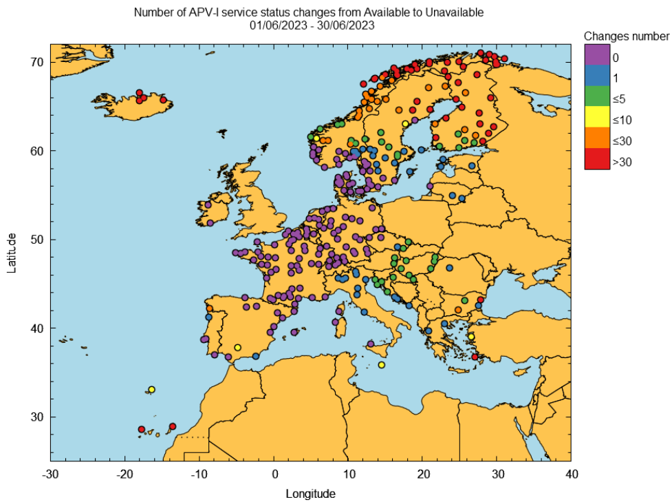
Figure 18 – EGNOS APV-I outages
