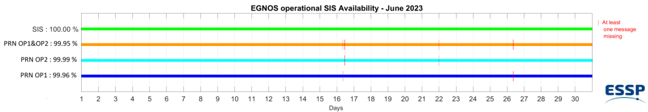
Figure 1 – EGNOS SIS & PRN Availability for June 2023
