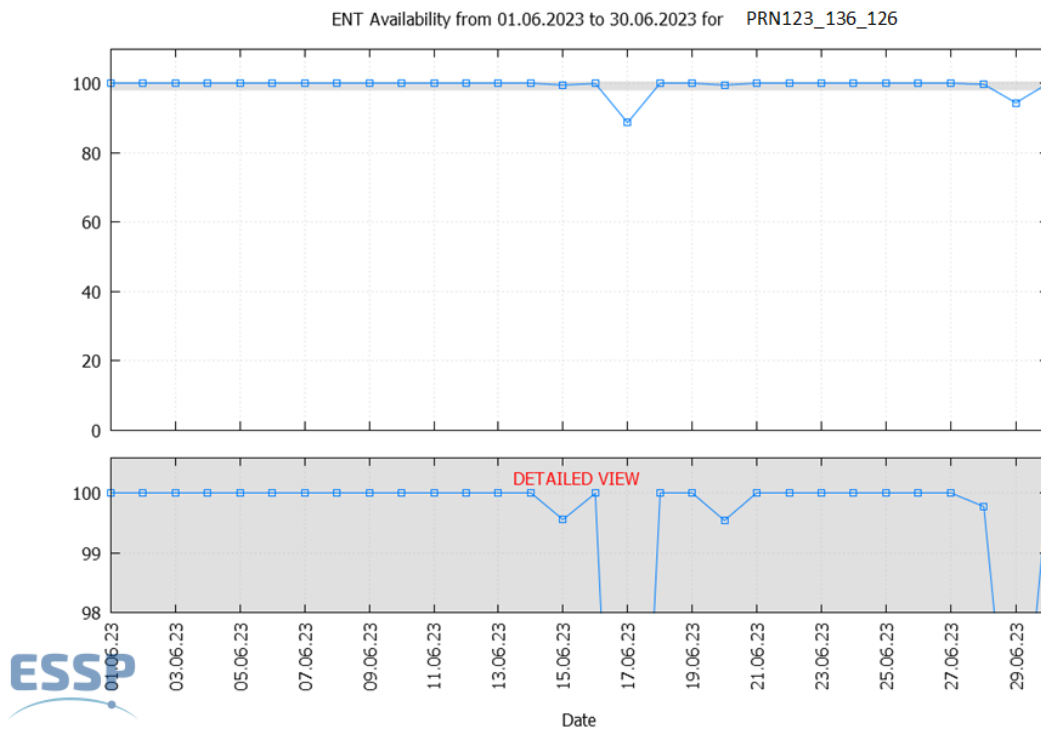
Figure 28 – EGNOS Time Service availability
