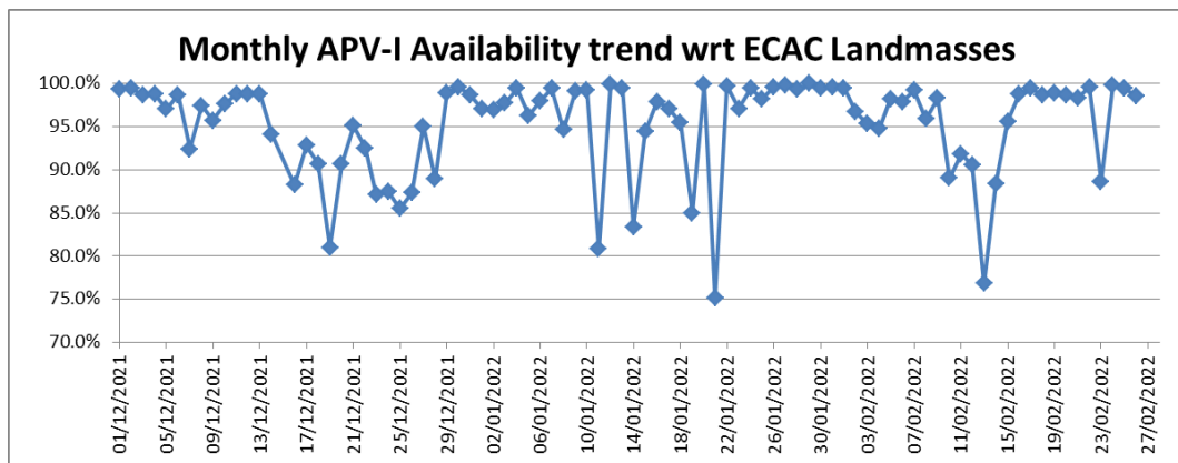
Figure 11 – EGNOS APV-I Availability compliance trend
