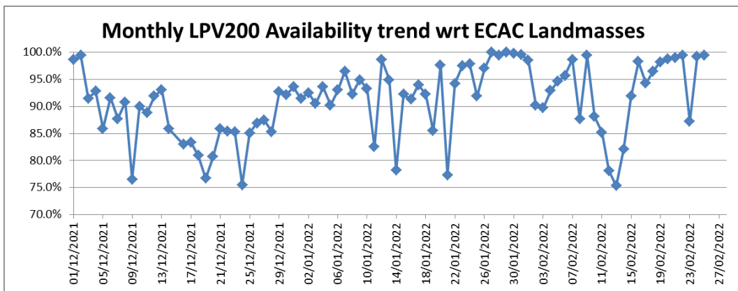
Figure 20 – EGNOS LPV-200 Availability compliance trend
