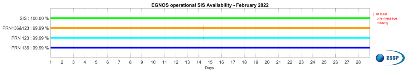
Figure 1 – EGNOS SIS & PRN Availability for February 2022
