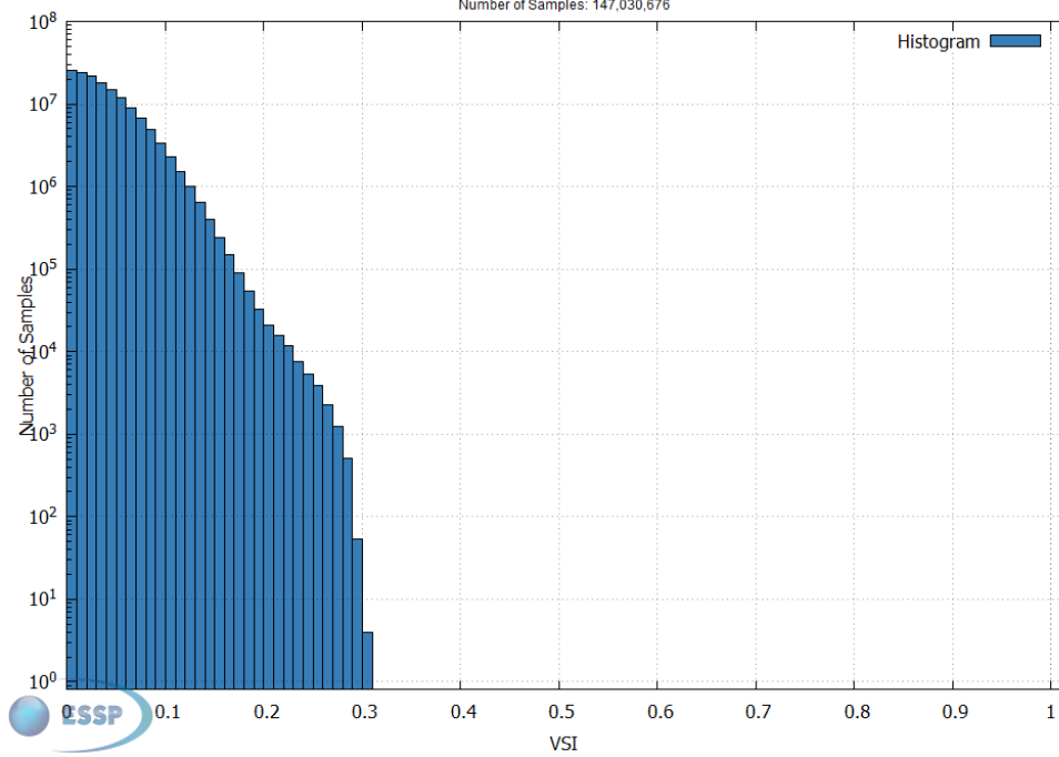
Figure 14 – EGNOS APV-I Vertical Safety Index of the month
